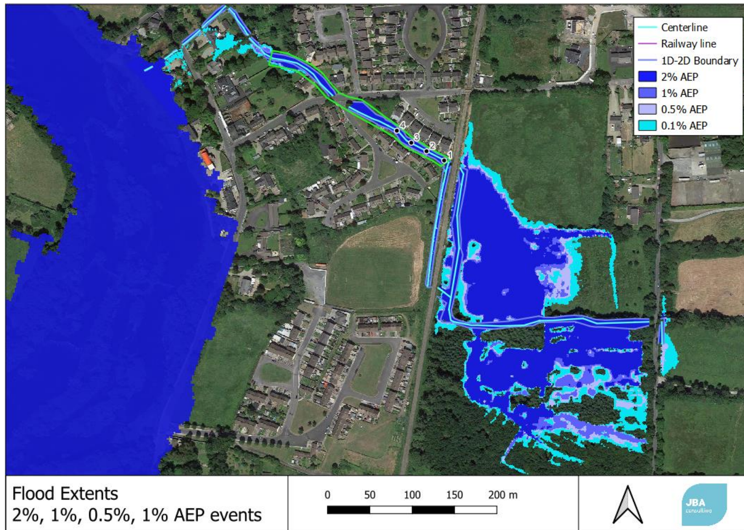
Figure D0-17: 2%, 1% 0.5%, 0.1% AEP Flood Extents
