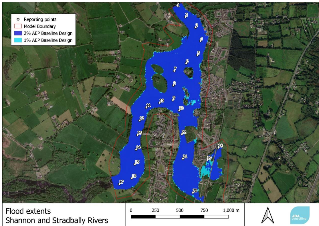
Figure B-7: Shannon and Stradbally Watercourses Flood Extents – 2% and 1% AEP Baseline Design Event (258 m 3 /s headrace flow)
