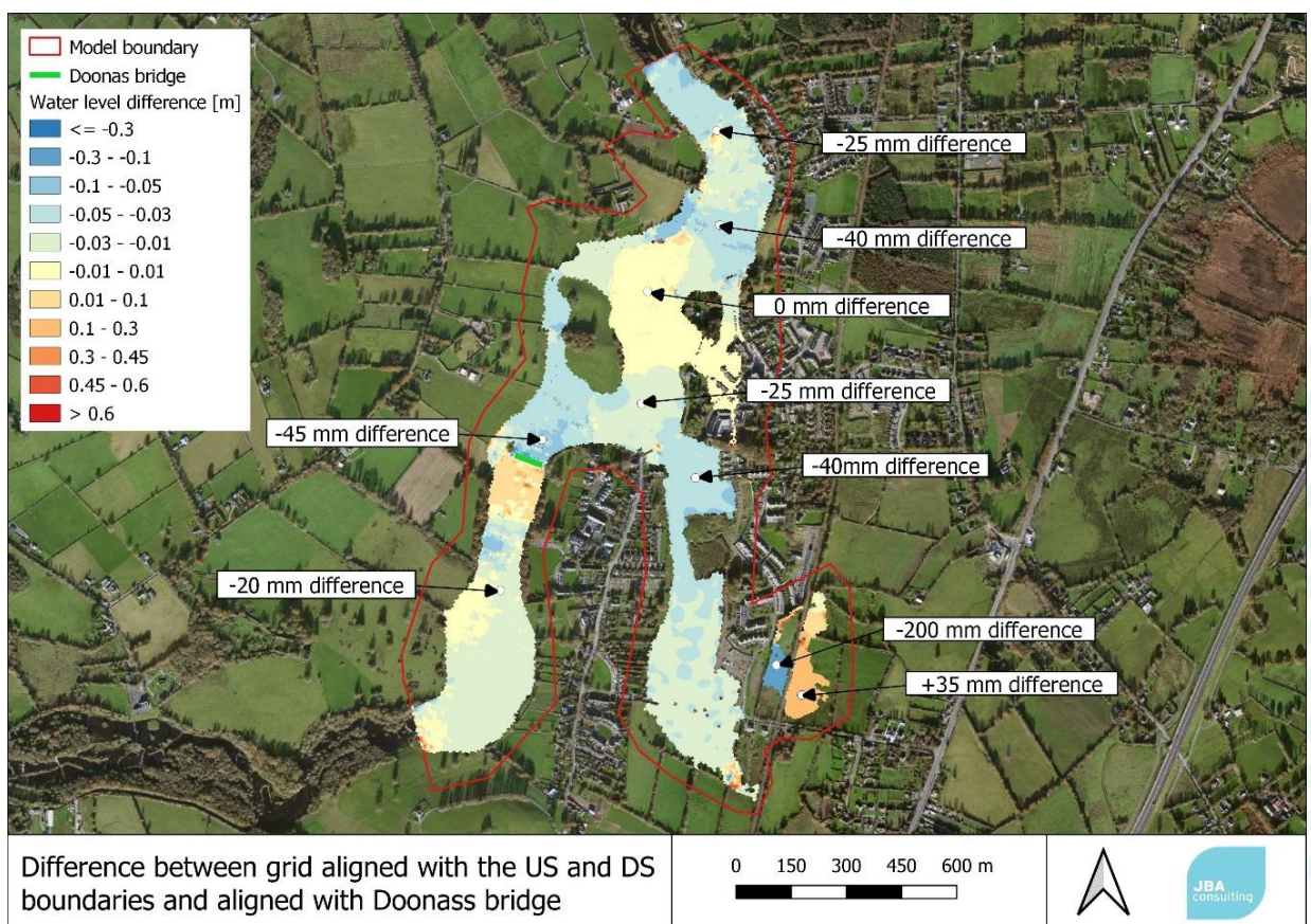
Figure 4-1: Grid orientation – water level difference (grid aligned with the US and DS boundaries - grid aligned with the Doonass Bridge)
