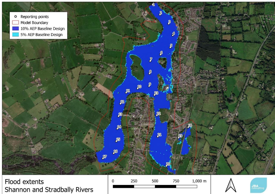
Figure B-6: Shannon and Stradbally Watercourses Flood Extents – 10% and 5% AEP Baseline Design Event (258 m 3 /s headrace flow)
