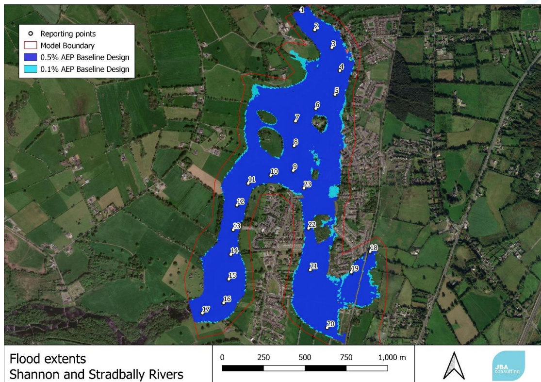
Figure B-8: Shannon and Stradbally Watercourses Flood Extents – 0.5% and 0.1% AEP Baseline Design Event (258 m 3 /s headrace flow)
