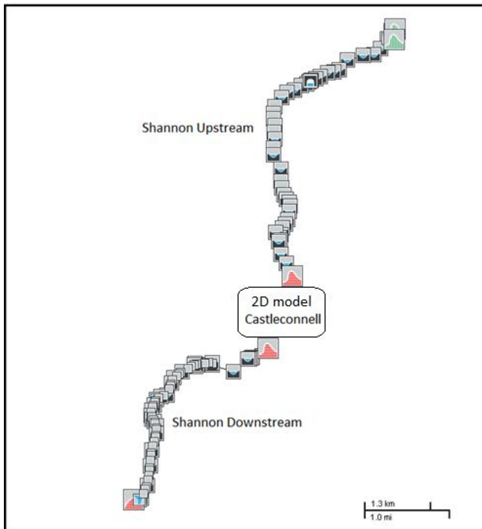
Figure 2-2: 1D Flood Modeller schematisation
