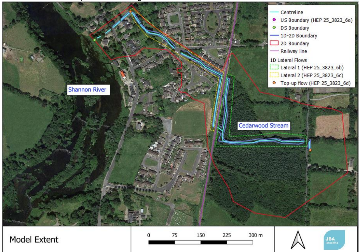
Figure D0-1: Model Extent
