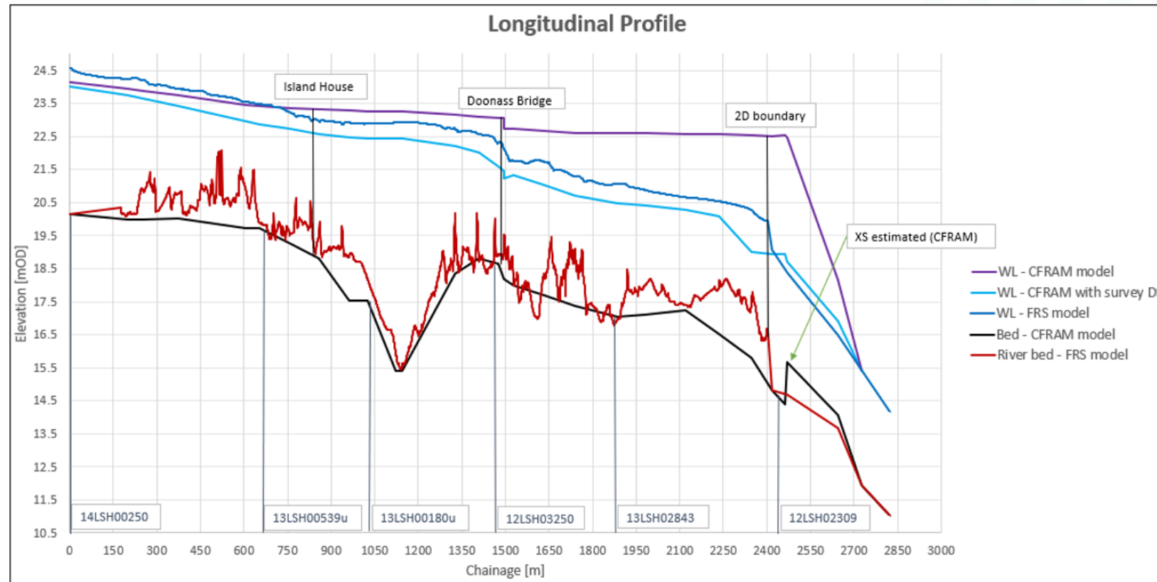
Figure 3-8: 1% AEP (with 345 m 3 /s headrace flow to Ardnacrusha) Longitudinal profile– FRS and CFRAM water levels
