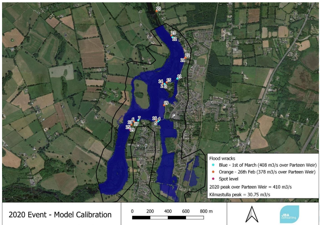
Figure 3-2: Model Calibration – 2020 event
