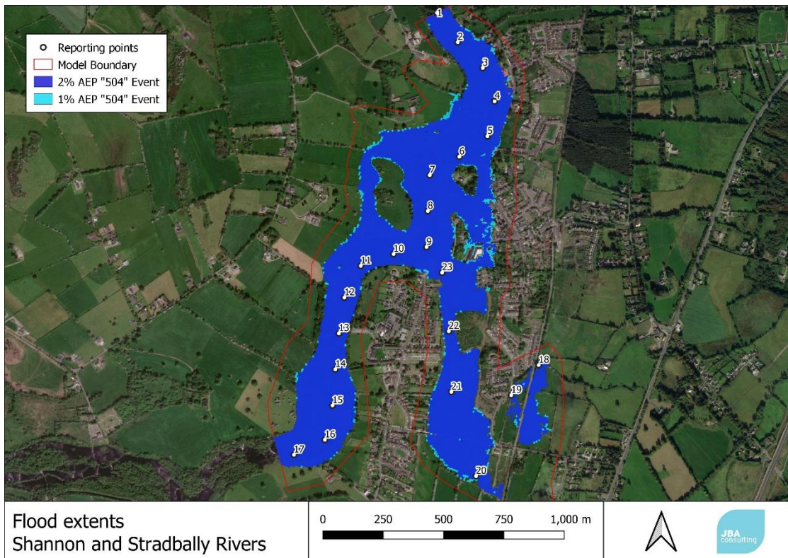
Figure B-3: Shannon and Stradbally Watercourses Flood Extents – 2% and 1% AEP "504" event (345 m 3 /s headrace flow)
