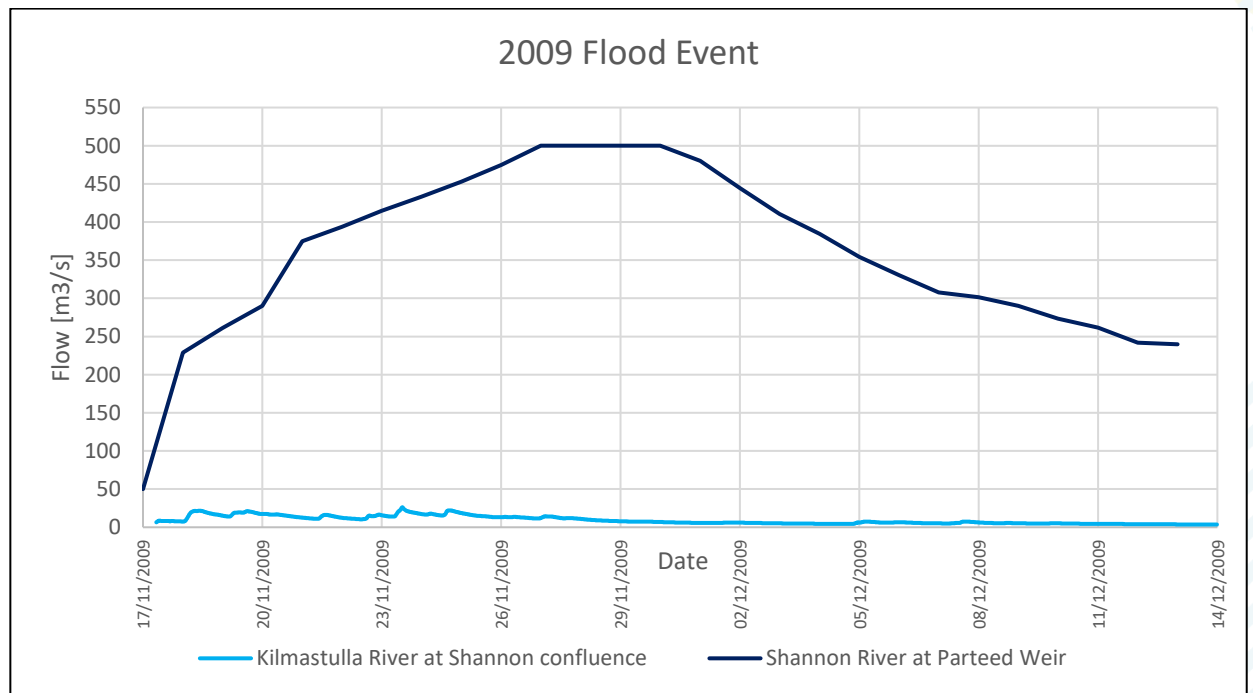
Figure 3-3: 2009 event – Flow Hydrograph
