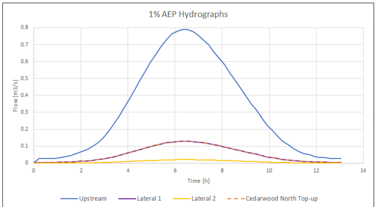
Figure D0-2: 1% AEP Hydrograph – Cedarwood Stream
