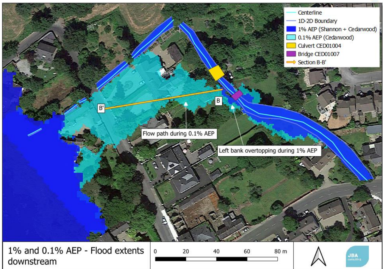
Figure D0-7: 1% AEP flood extent - downstream end of Cedarwood Stream
