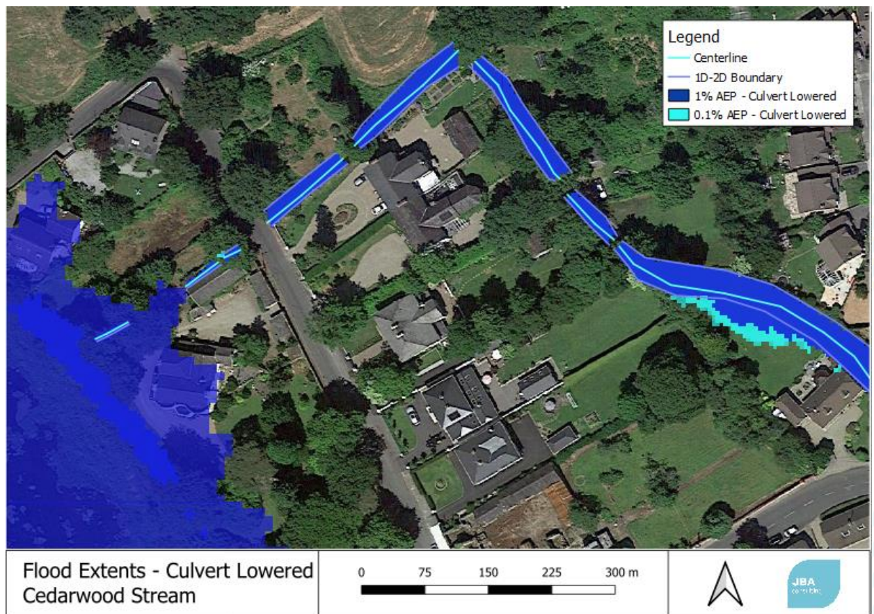
Figure D0-20: 1% and 0.1% AEP Flood Extents – “Culvert Lowered” Scenario
