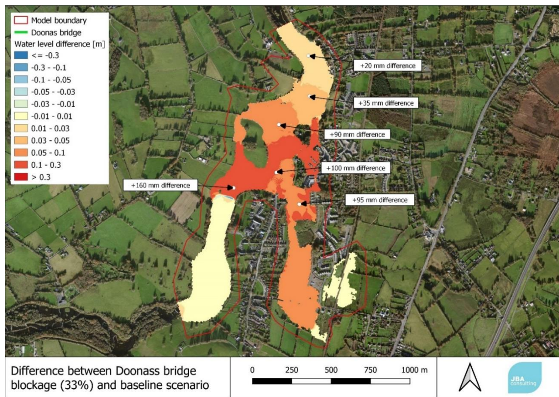
Figure 4-8: Difference between blockage scenario (33%) and baseline scenario (blockage scenario – baseline scenario)
