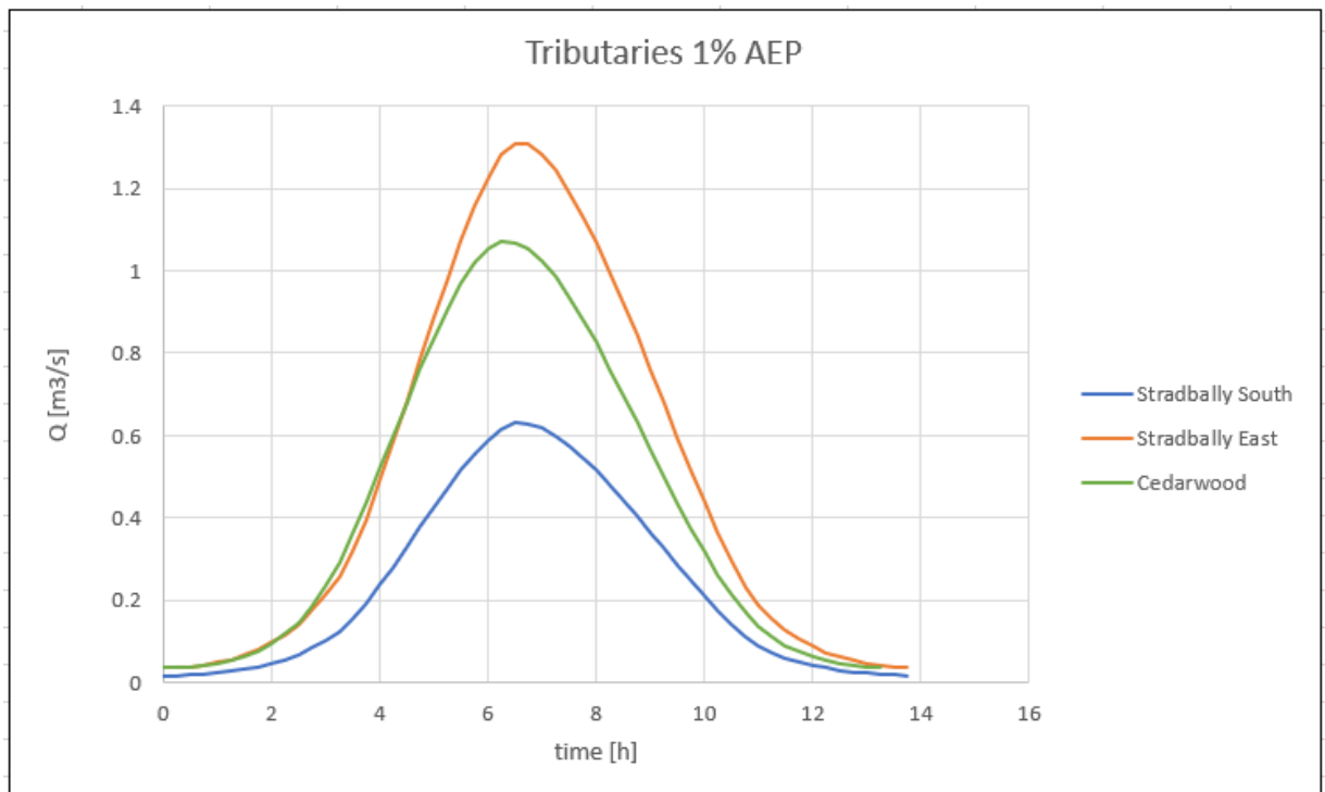
Figure 2-7: Cedarwood and Stradbally Streams 1% AEP
