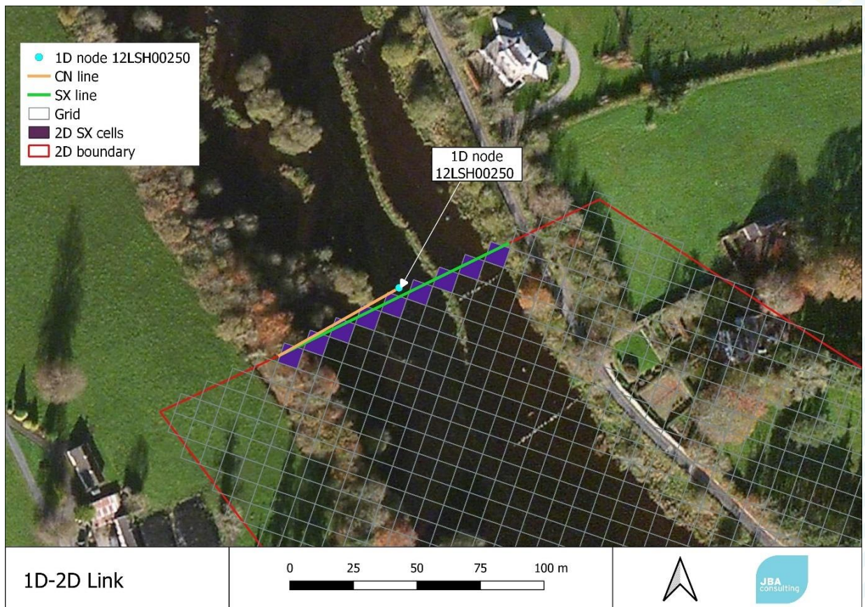
Figure 2-10: Linking between 1D and 2D models
