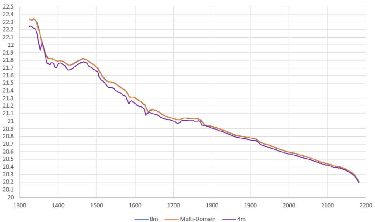
Figure 4-6 Longitudinal profile – Downstream of Doonass Bridge
