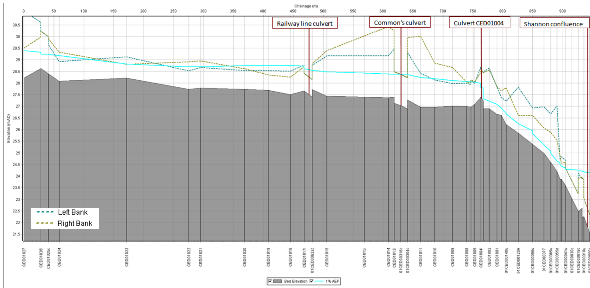
Figure D0-10: Cedarwood Stream - Peak 1% Water Level – Longitudinal Section
