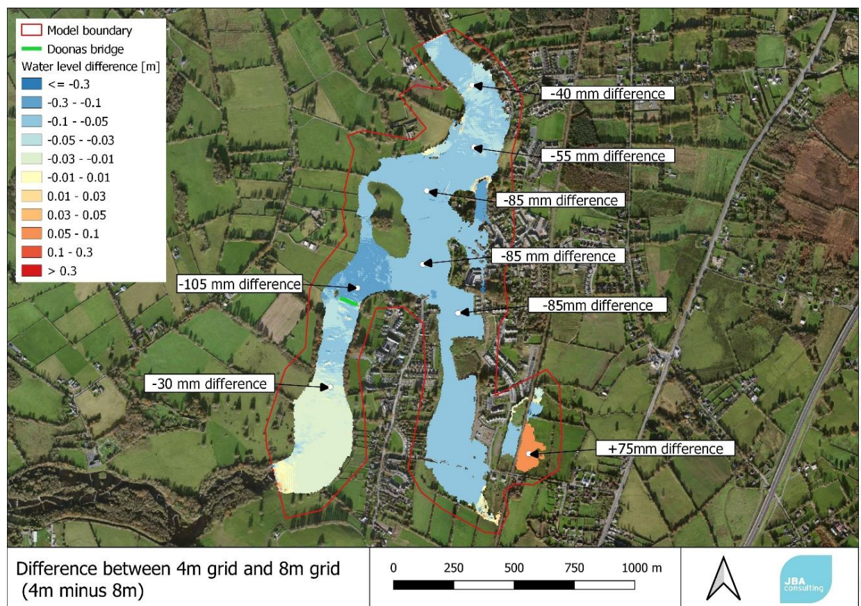
Figure 4-2: Difference between 4m and 8m scenario (4m minus 8m scenario)
