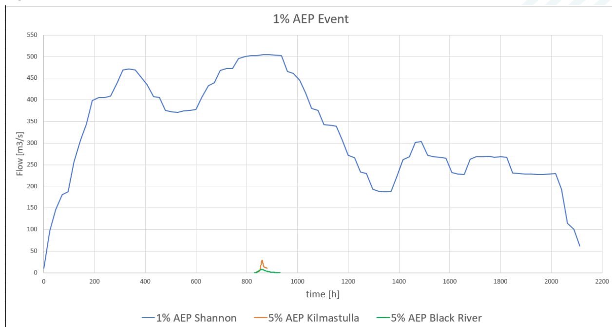
Figure 2-5: Old Shannon downstream of Parteen Weir 1% AEP (after headrace flow of 345 m³/s to Ardnacrusha – “504 event”)
