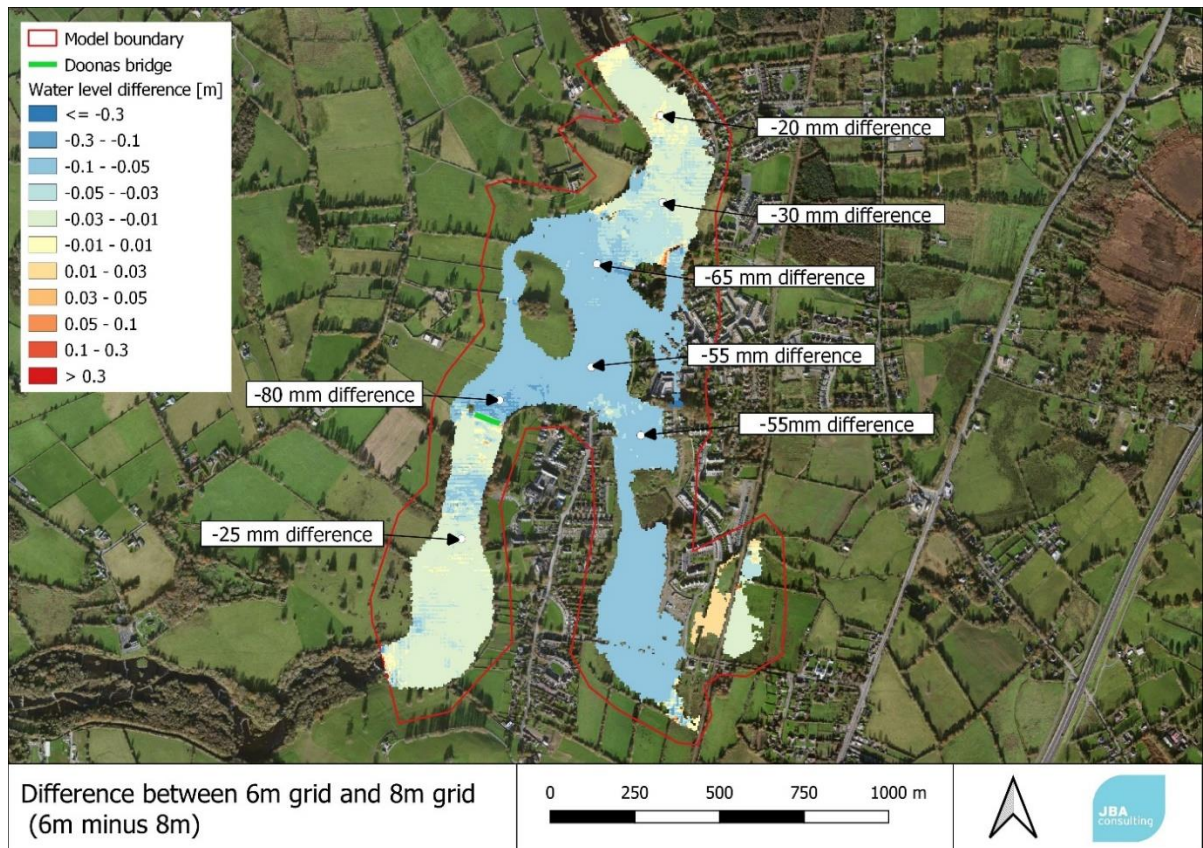
Figure 4-3: Difference between 6m and 8m scenario (6m minus 8m scenario)
