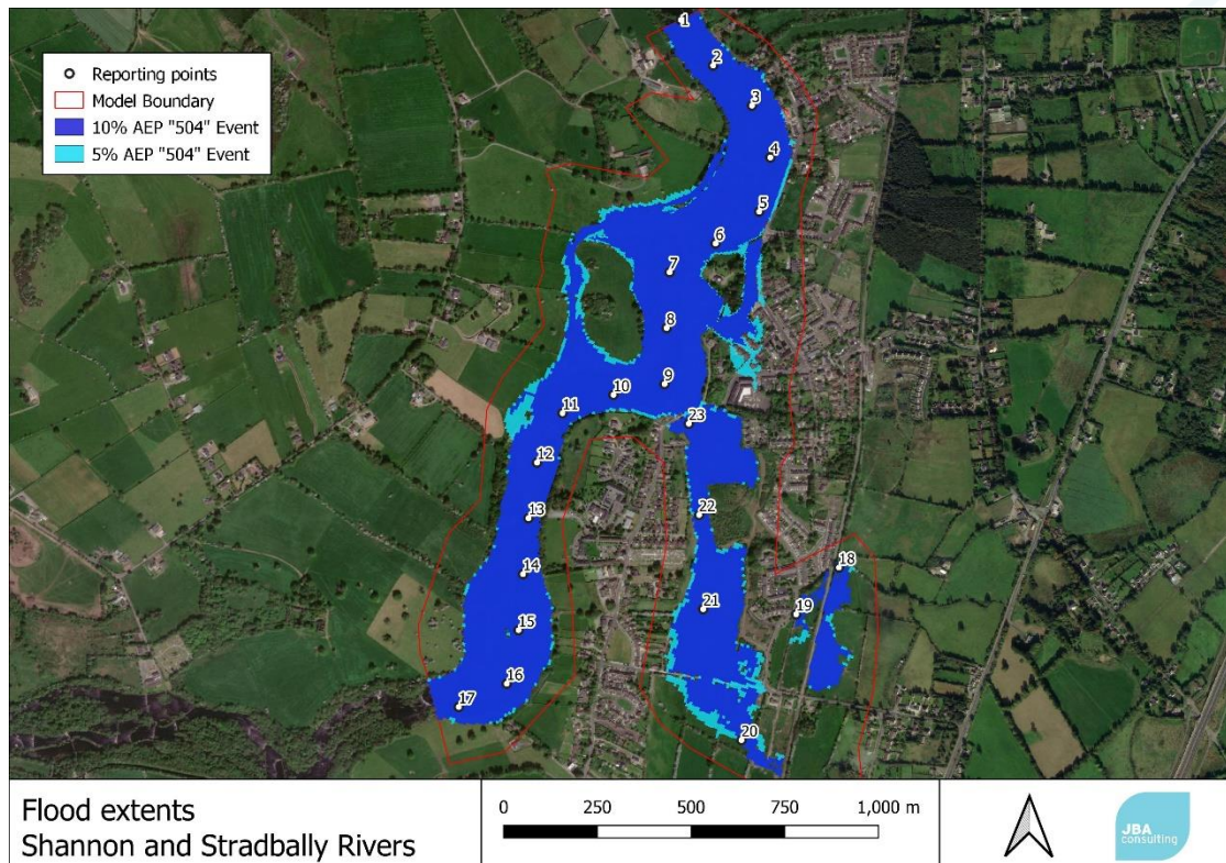
Figure B-2: Shannon and Stradbally Watercourses Flood Extents – 10% and 5% AEP "504" event (345 m³/s headrace flow)
