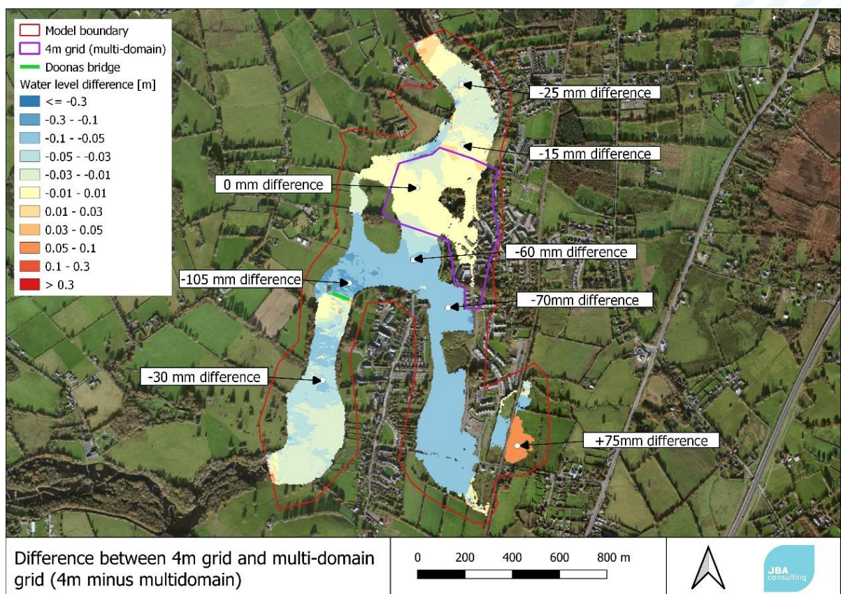
Figure 4-4 Difference between 4m and multi-domain scenario (4m minus multi-domain scenario)
