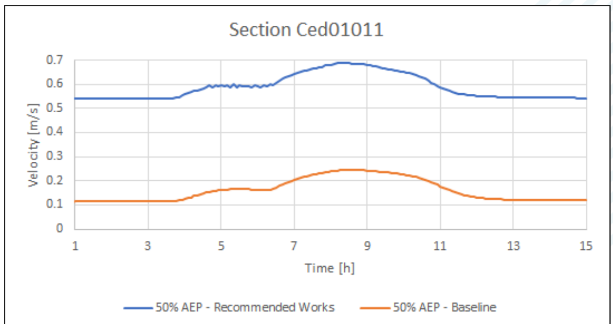
Figure D0-28: 50% AEP Velocities – Section Ced01011 (Downstream of Common's Road)
