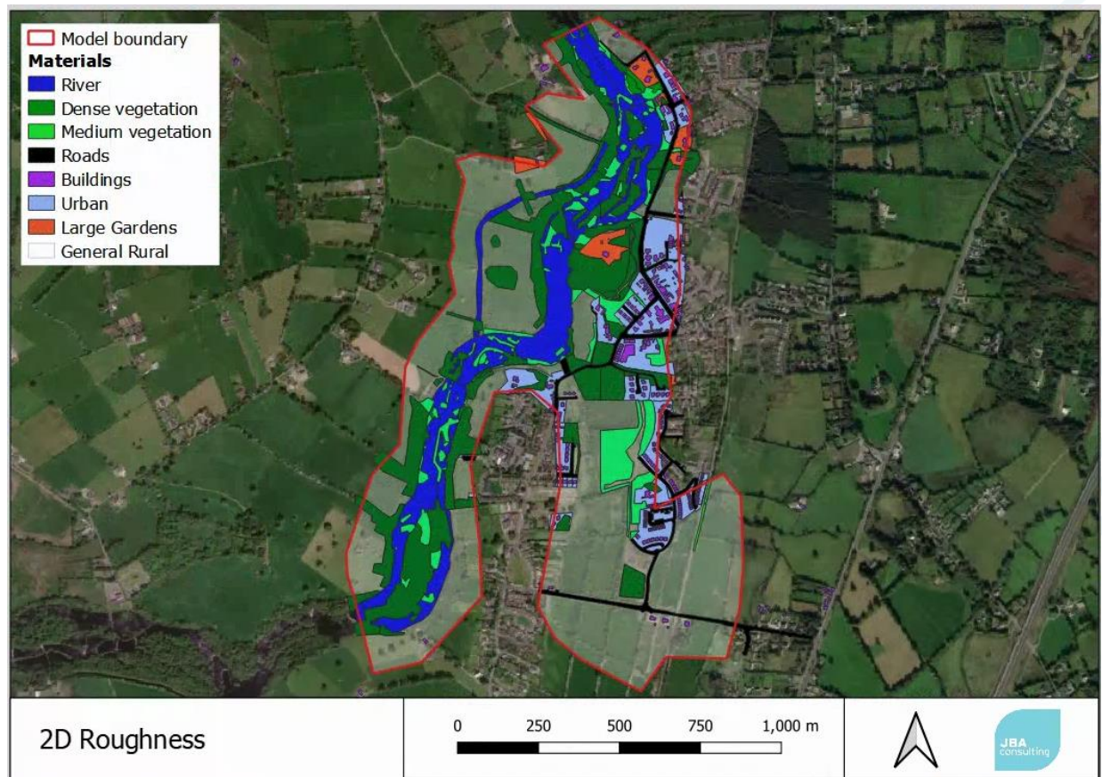
Figure 2-18: Materials layer – Spatial distribution
