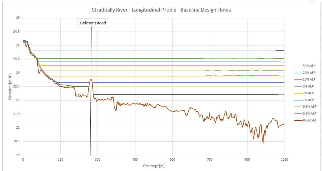
Figure B-14: Stradbally Stream – Longitudinal Profile – Baseline Design Event (258 m 3 /s headrace flow)
