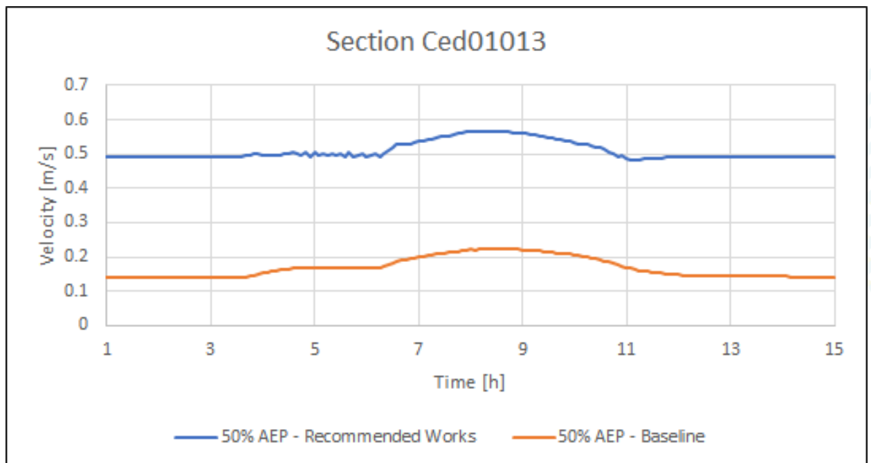
Figure D0-27: 50% AEP Velocities – Section Ced01013 (Cedarwood Grove)
