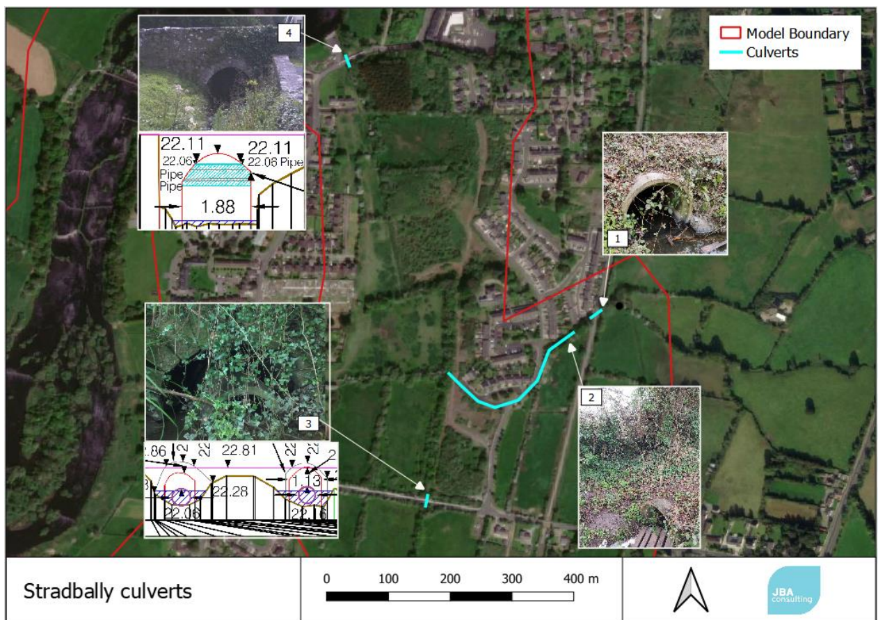
Figure 2-26: Stradbally culverts
