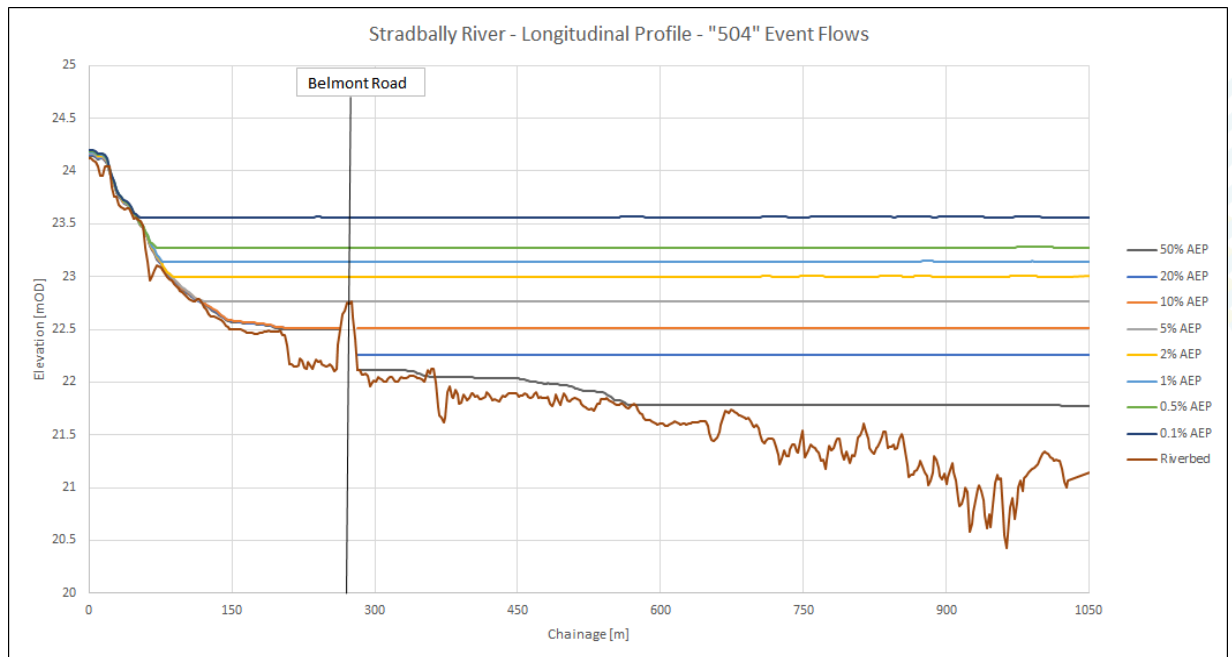
Figure B-13: Stradbally Stream – Longitudinal Profile "504" event (354 m 3 /s headrace flow)
