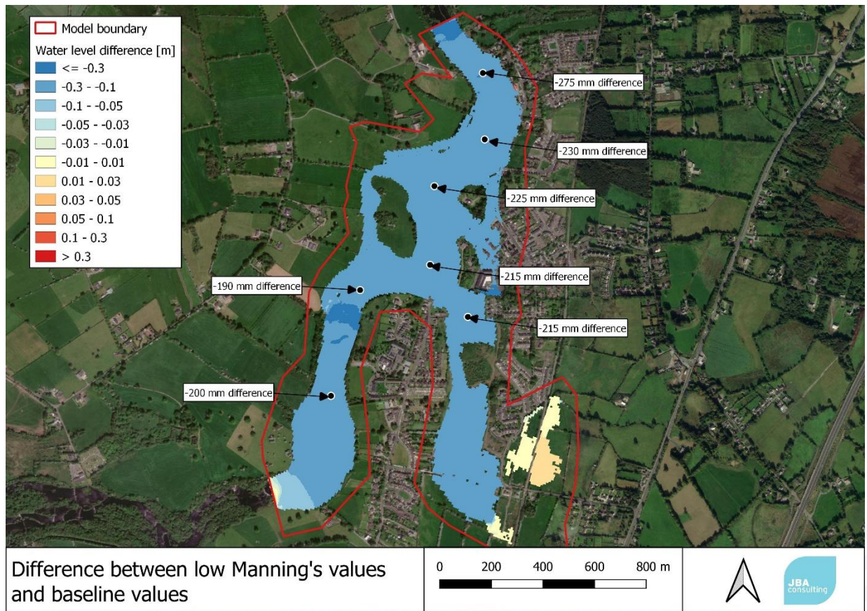
Figure 4-15: Difference between low Manning's n values and baseline scenario (low Manning's minus baseline values)
