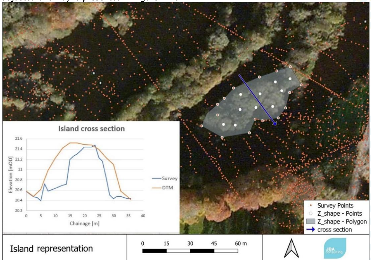
Figure 2-20: Island representation
