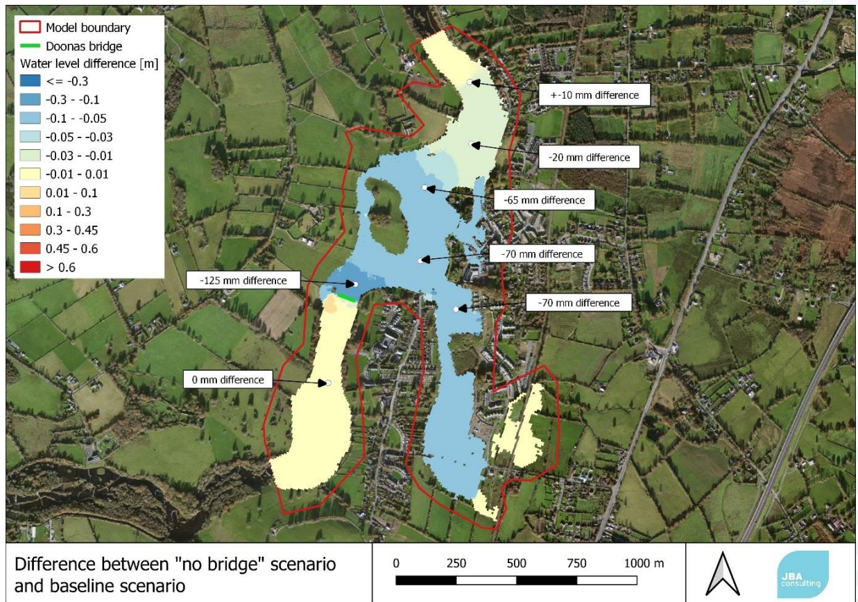
Figure 4-7: Difference between “No bridge” scenario and baseline scenario – “504” Event (“no bridge” scenario minus baseline scenario)
