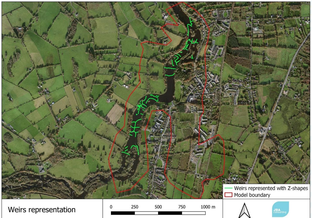
Figure 2-21: Weir Representation – Plan View
