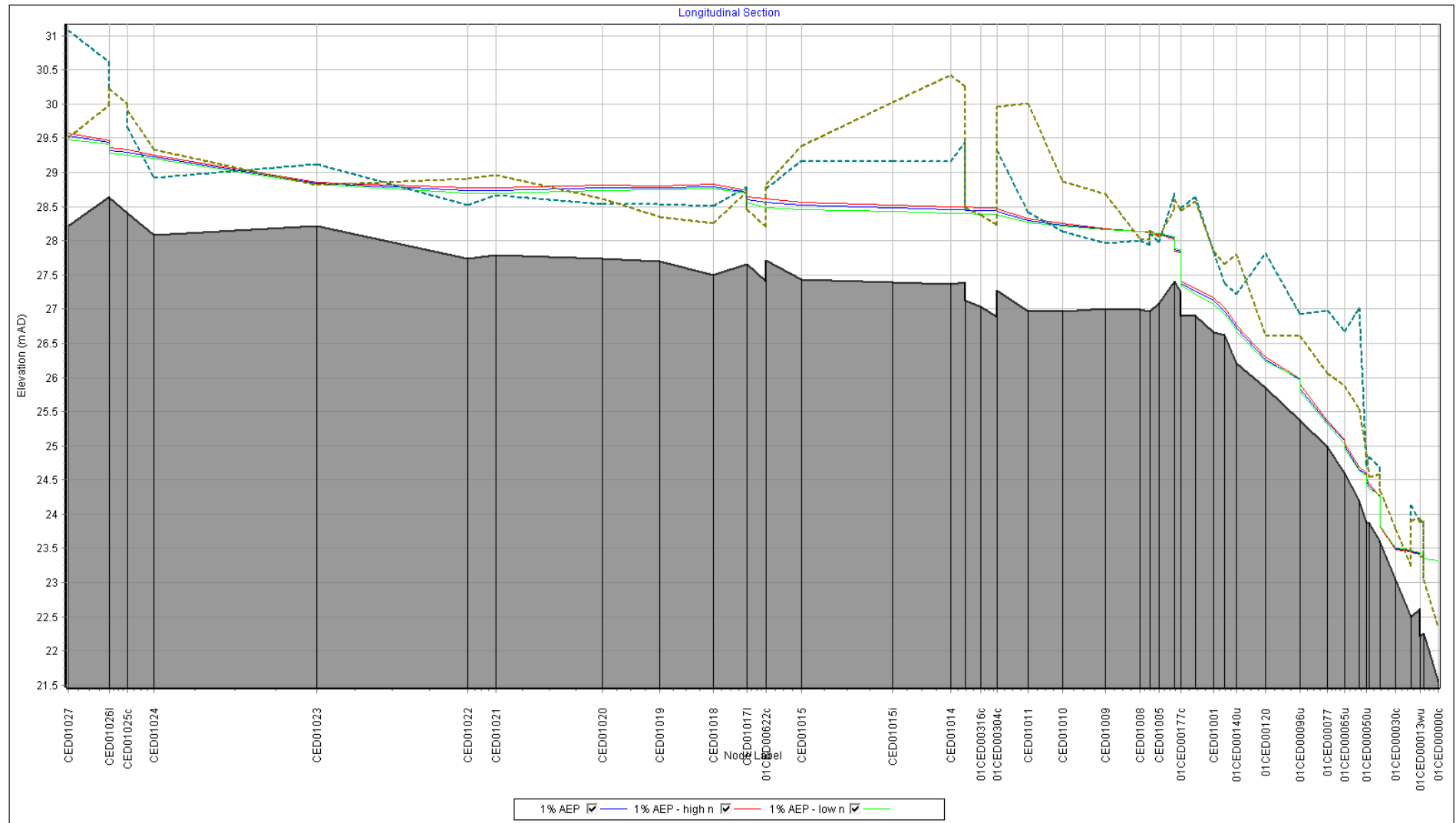
Figure D0-11: Cedarwood Stream - Peak 1% Water Level – Longitudinal Section high & low Manning's n
