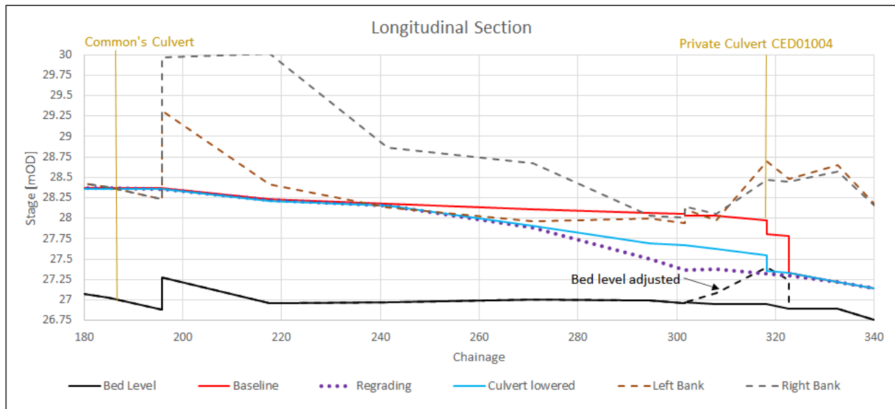
Figure D0-21: Longitudinal Section – Culvert Testing
