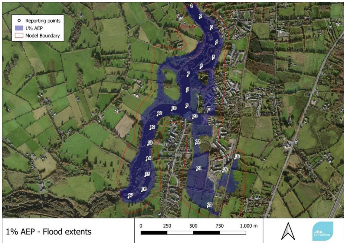
Figure 5-1: 1% AEP for “504” event (345 m 3 /s headrace flow)
