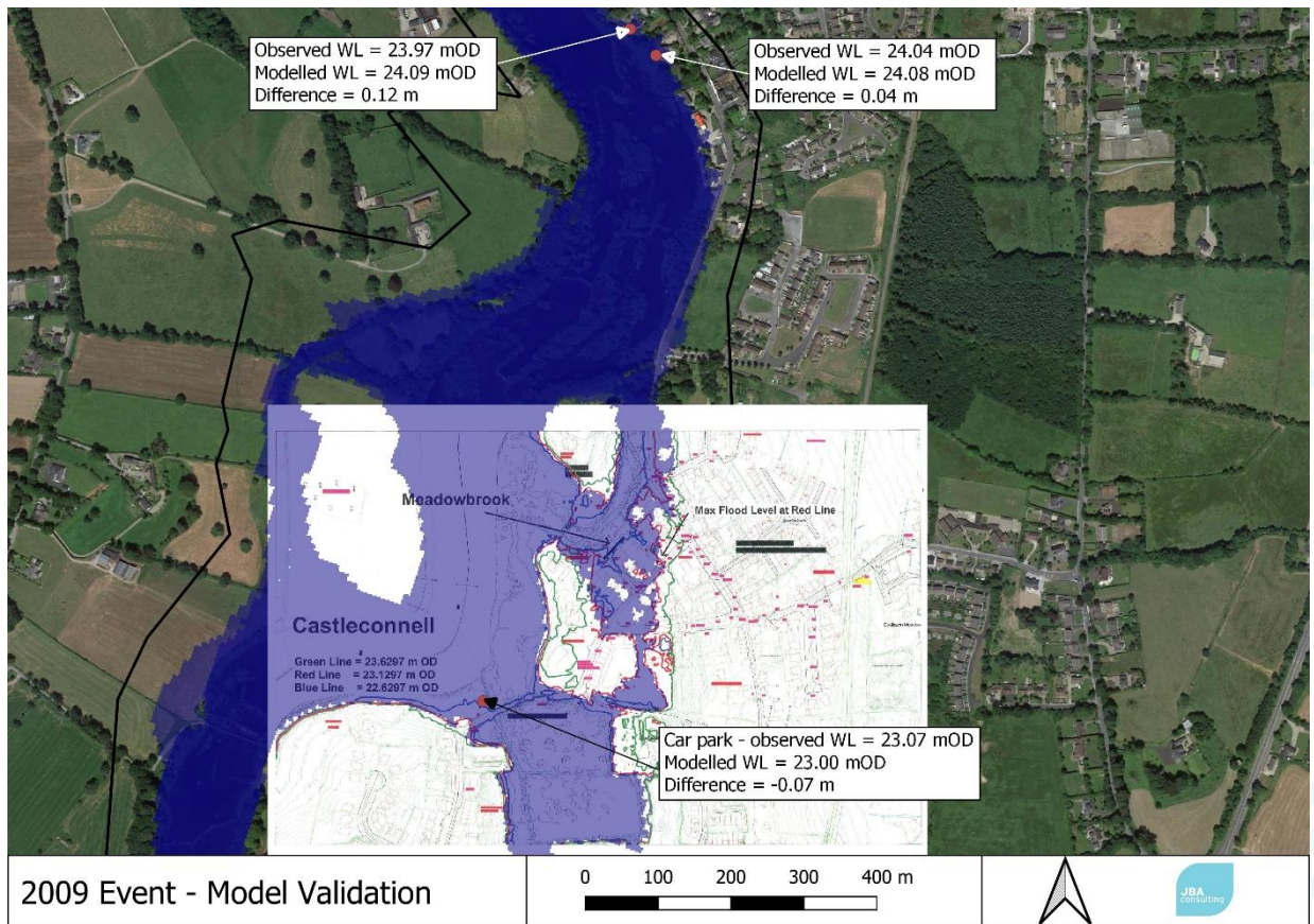
Figure 3-4: Model Validation – 2009 Event
