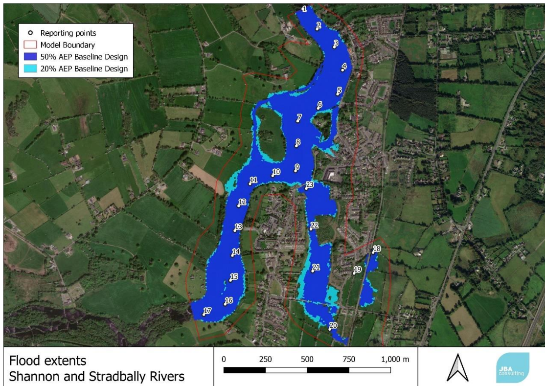
Figure B-5: Shannon and Stradbally Watercourses Flood Extents – 50% and 20% AEP Baseline Design Event (258 m 3 /s headrace flow)
