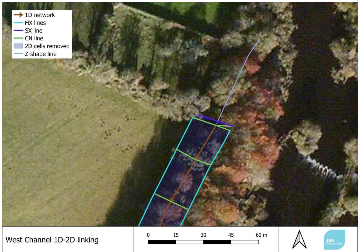
Figure 2-24: West Channel 1D-2D link
