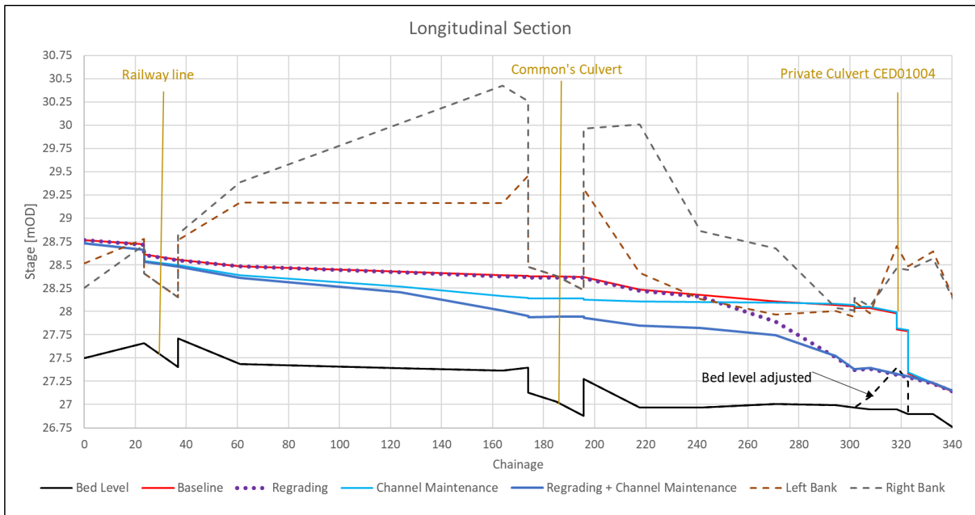
Figure D0-23 –Longitudinal Section - 1% AEP Peak Water Levels
