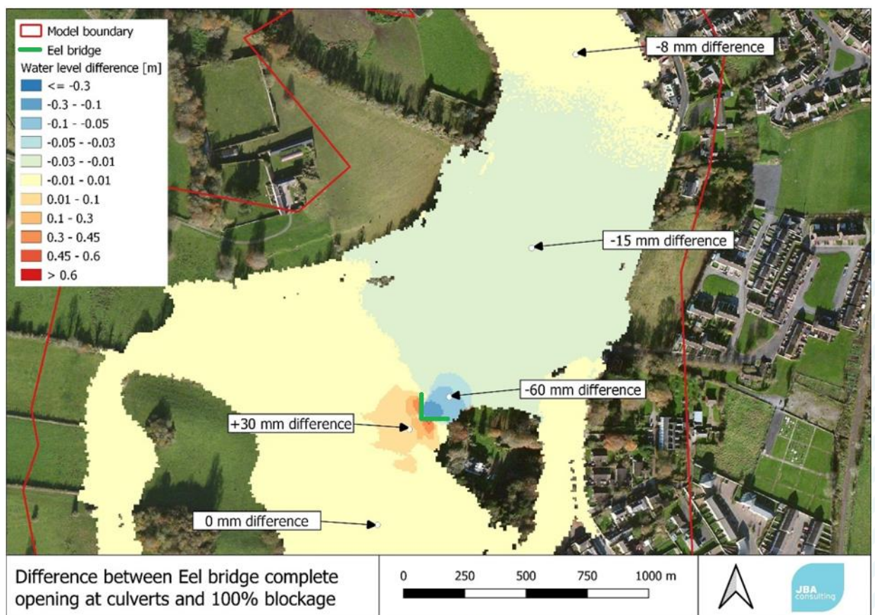
Figure 4-12: Difference between Eel bridge failure scenario and bridge blockage (100%) scenario (failure scenario minus blockage scenario)
