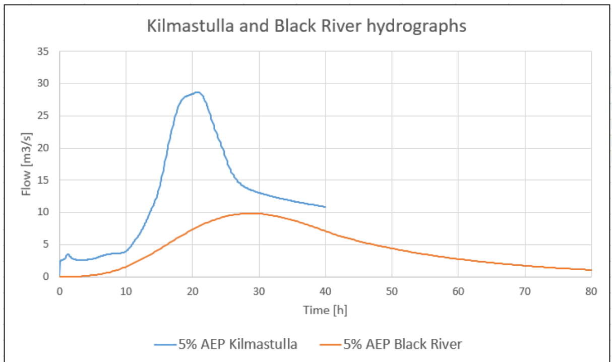
Figure 2-6: Kilmastulla and Black River 5% AEP
