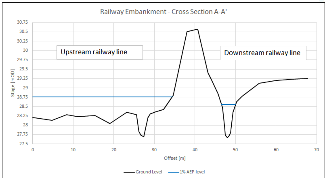
Figure D0-3: Railway Embankment – Cross Section A-A'
