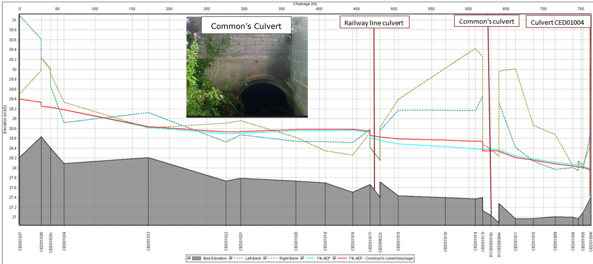
Figure D0-13: 1% AEP Longitudinal Section – Common's Road culvert blockage
