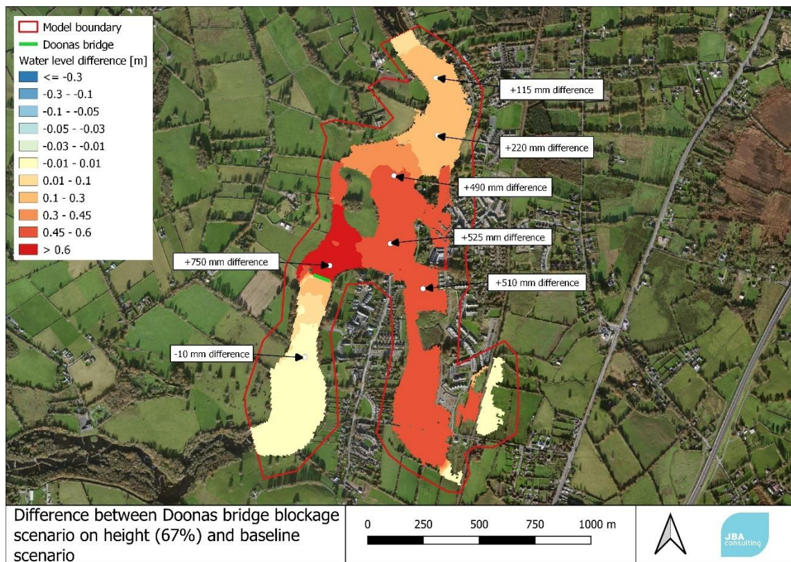
Figure 4-11: Difference between bridge blockage on height (67%) and baseline scenario (blockage scenario – baseline scenario)
