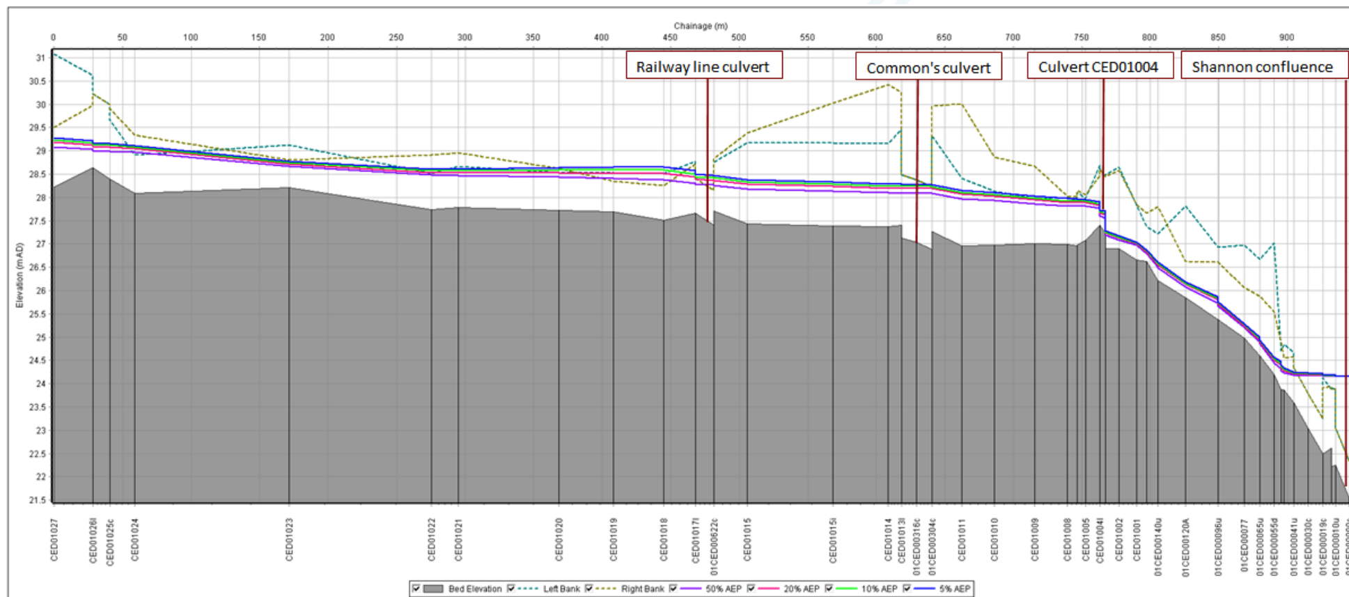
Figure D0-18: Water Levels 5%, 10%, 20% and 50% AEP Events – Longitudinal Section
