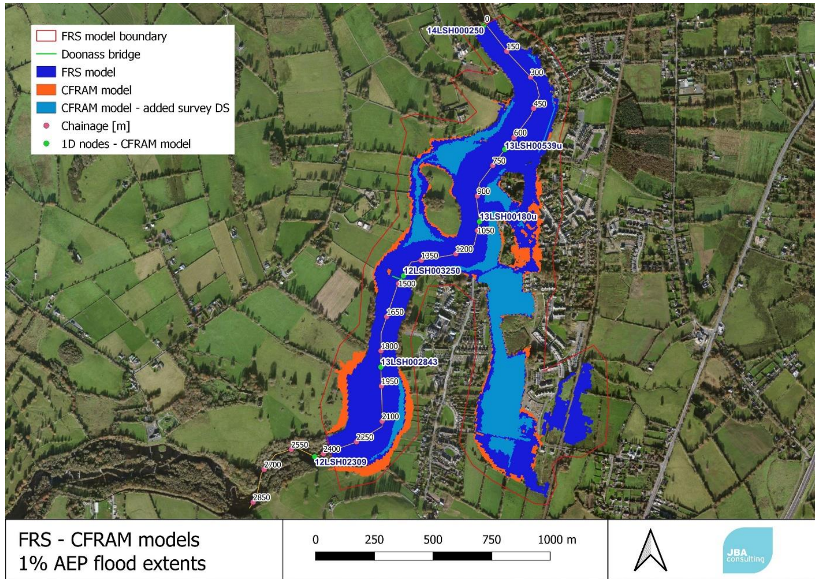
Figure 3-7: 1% AEP Flood extents – FRS and CFRAM models
