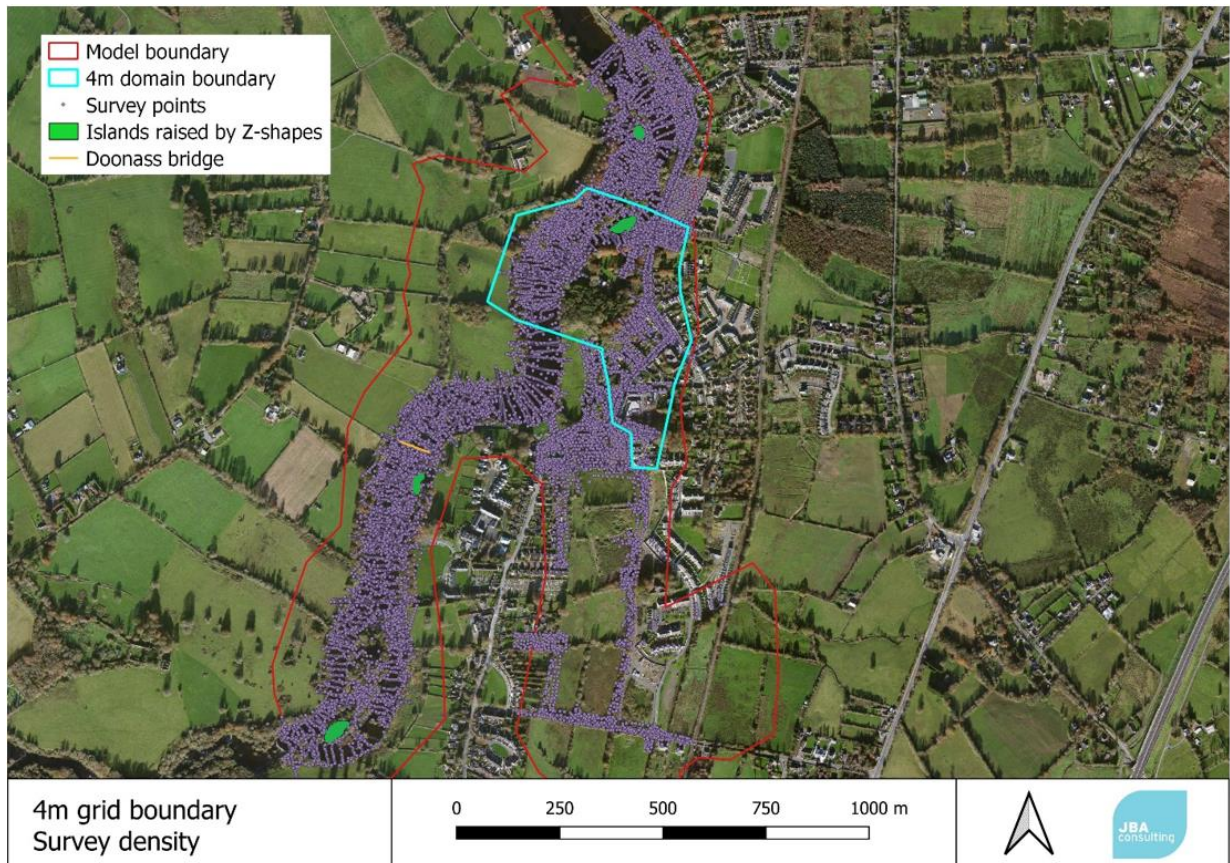
Figure 2-16: 4m grid boundary. Survey density
