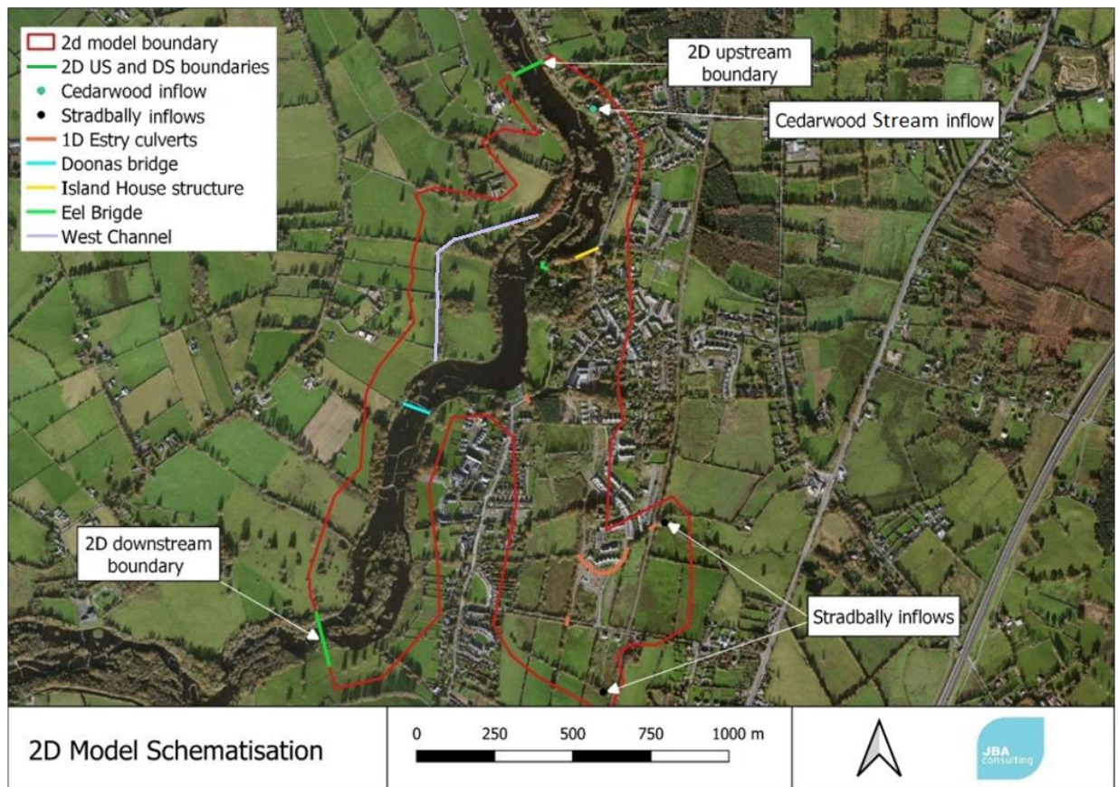
Figure 2-3: 2D Model Schematisation
