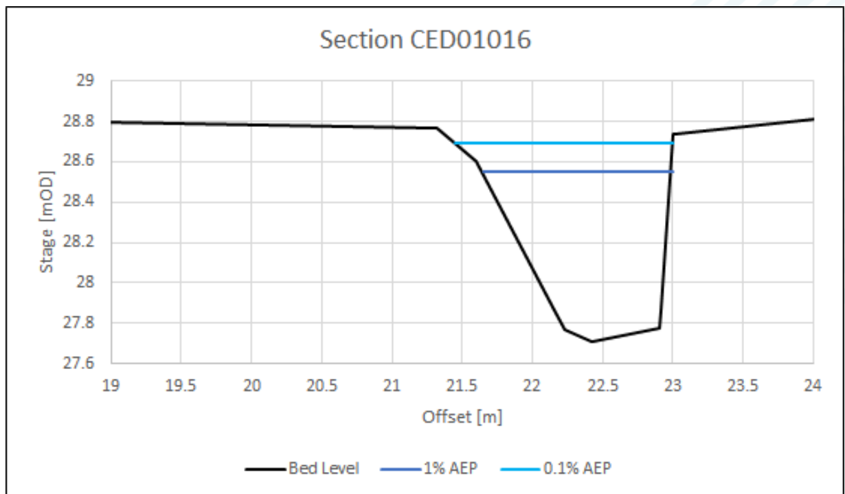
Figure D0-6: 1% and 0.1% AEP water levels – Section CED01016 at Cedarwood Grove
