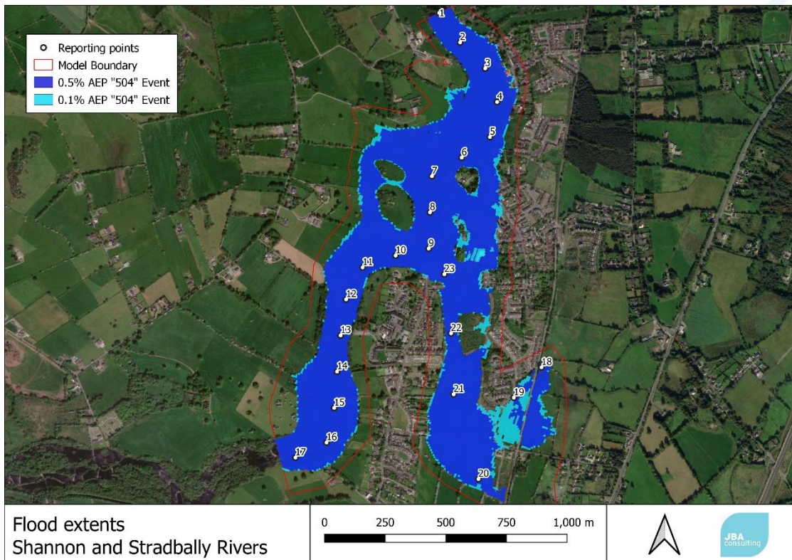
Figure B-4: Shannon and Stradbally Watercourses Flood Extents – 0.5% and 0.1% AEP "504" event (345 m 3 /s headrace flow)
