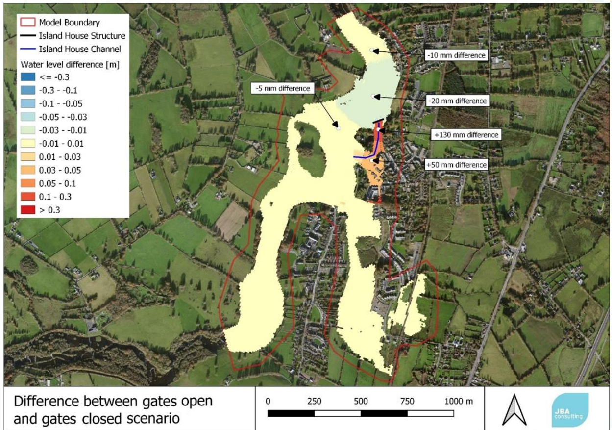
Figure 4-13: Difference between flood gates open and flood gates closed scenarios (flood gates open scenario minus flood gates closed scenario)
