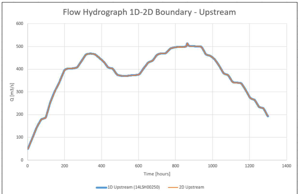
Figure 2-11: Flow Hydrographs Modelled at the Upstream 1D-2D Boundary (1% AEP with 345 m 3 /s headrace flow – “504 event”)
