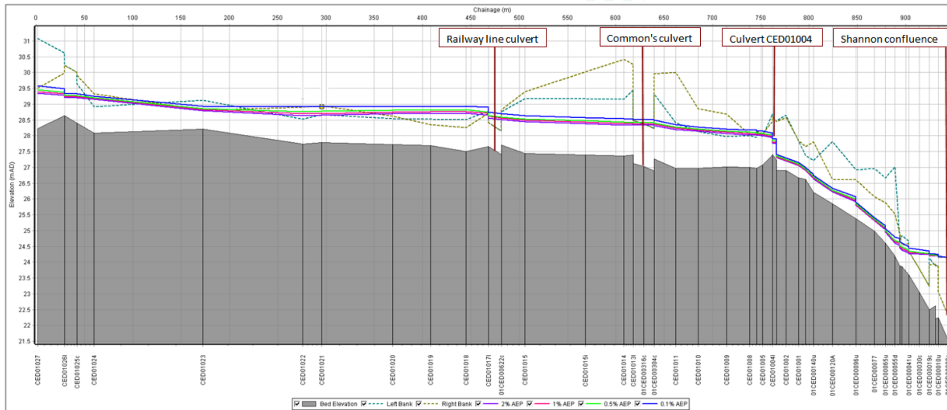
Figure D0-19: Water Levels 0.1%, 0.5%, 1% and 2% AEP Events – Longitudinal Section
