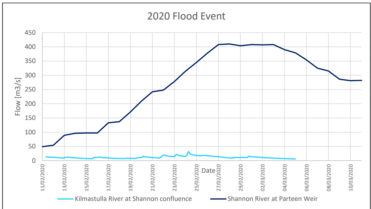
Figure 3-1: 2020 event – Flow Hydrograph
