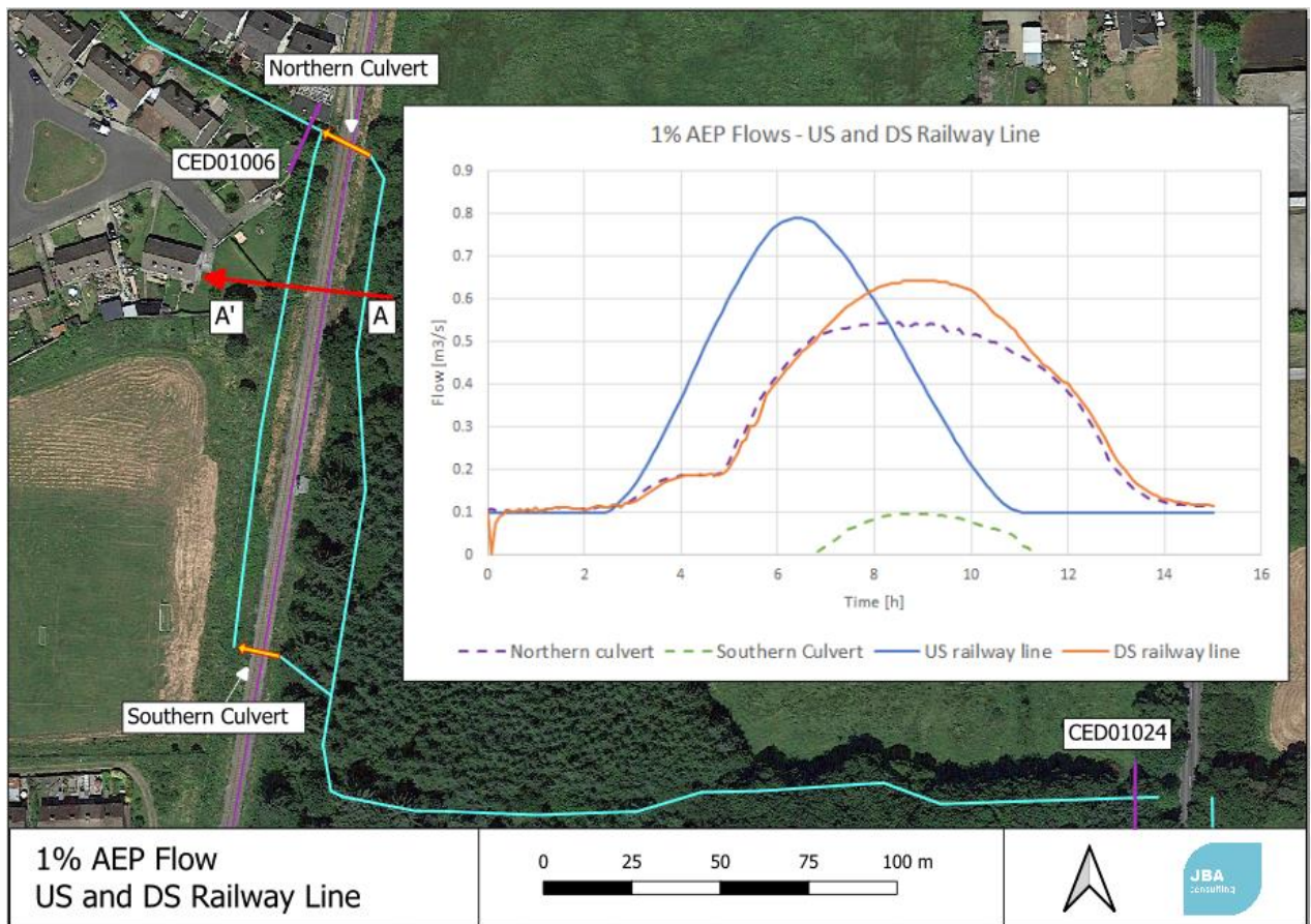
Figure D0-4: 1% AEP Hydrographs upstream and downstream of the railway line
