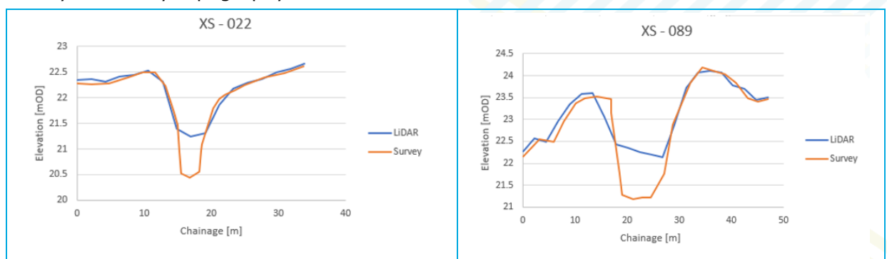
Figure 2-23: Topo-survey difference – cross sections
