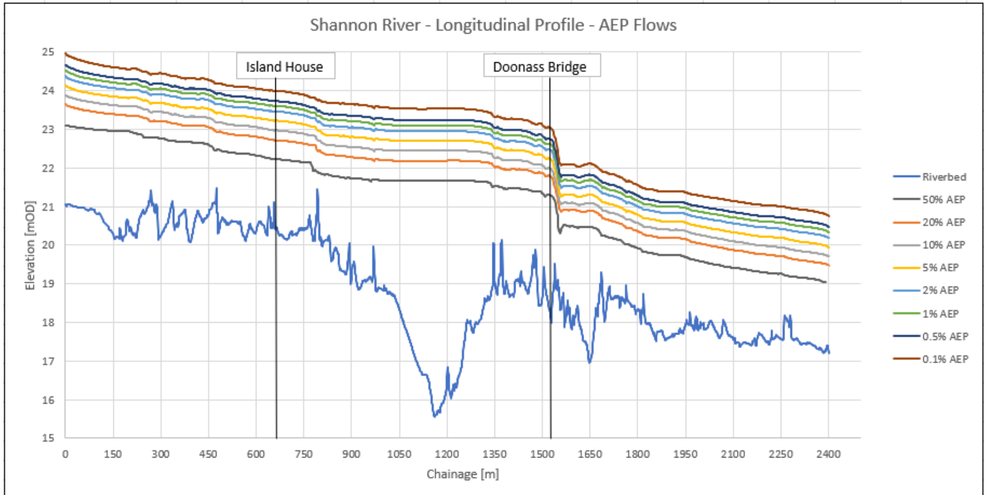
Figure B-10: Shannon River – Longitudinal Profile – “504” event (345 m 3 /s headrace flow)
