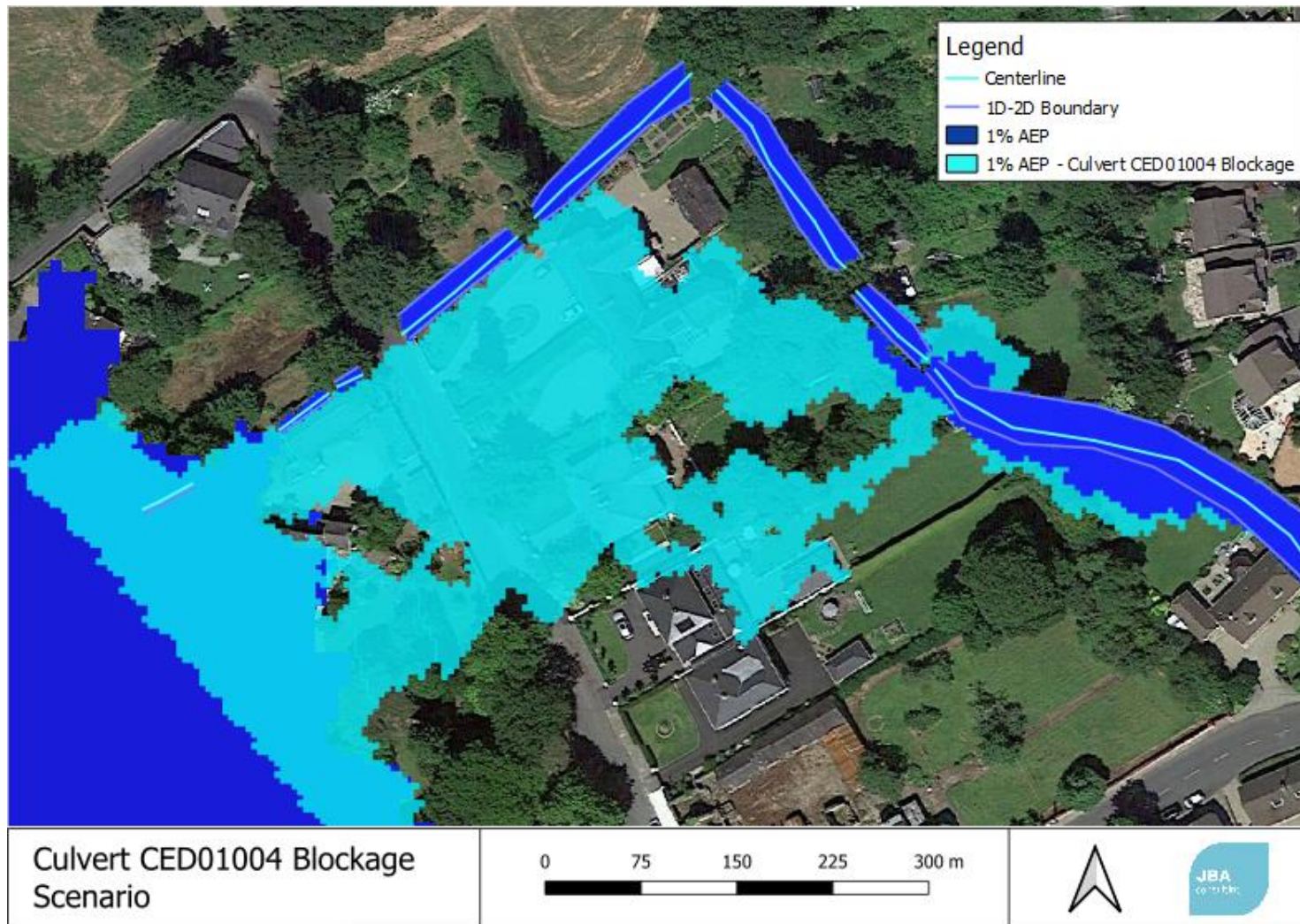
Figure D0-15: 1% AEP – Culvert CED01004 Blockage Scenario
