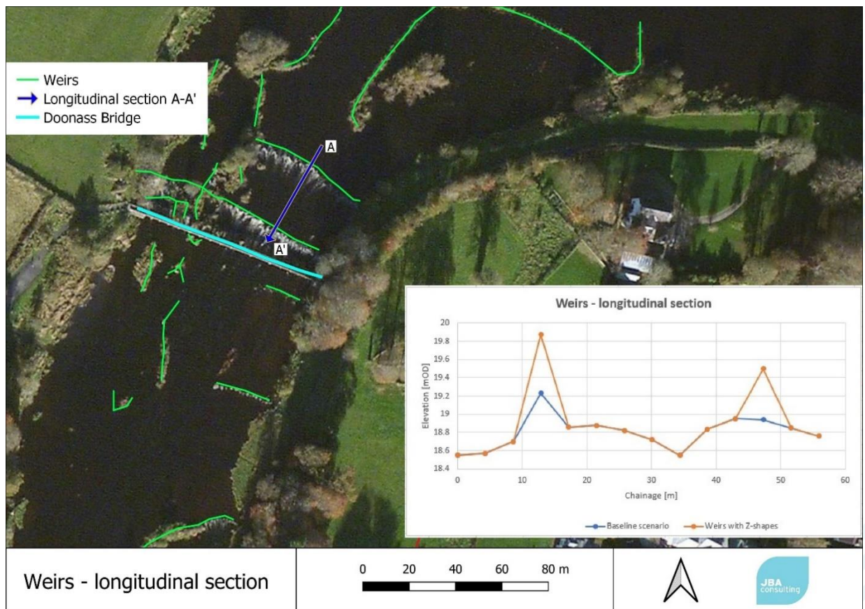
Figure 2-22: Weir representation – Longitudinal section
