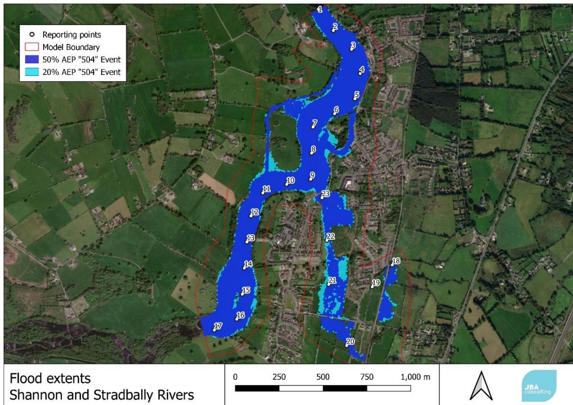
Figure B-1: Shannon and Stradbally Watercourses Flood Extents – 50% and 20% AEP "504" event (345 m³/s headrace flow)
