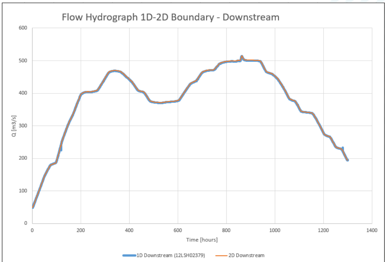
Figure 2-12: Flow Hydrographs Modelled at the Downstream 1D-2D Boundary (1% AEP with 345 m 3 /s diversion – “504 event”)
