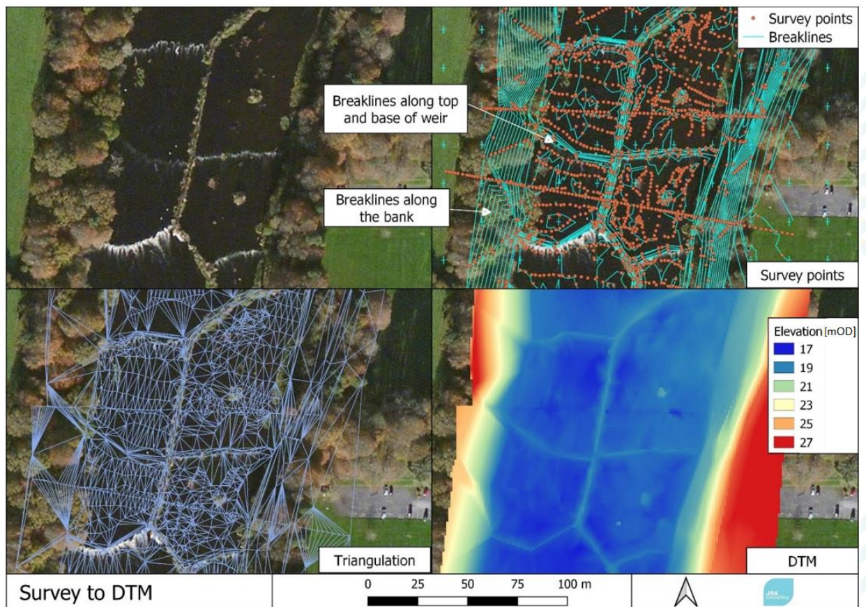
Figure 2-15: DTM generation from survey data
