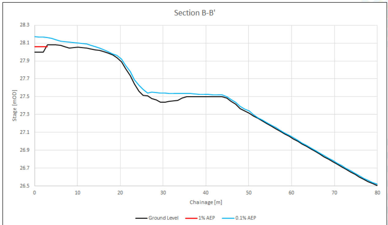
Figure D0-8: Section B-B' – 1% and 0.1% AEP levels
