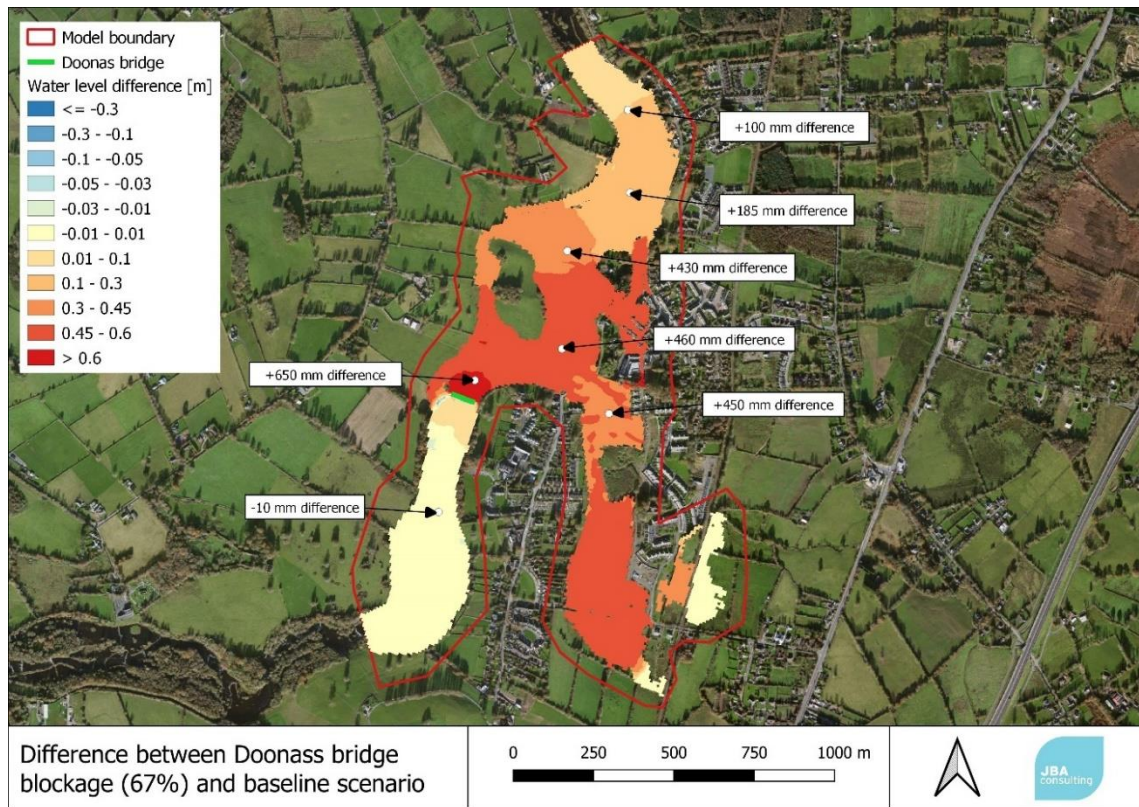
Figure 4-9: Difference between blockage scenario (67%) and baseline scenario (blockage scenario – baseline scenario)
