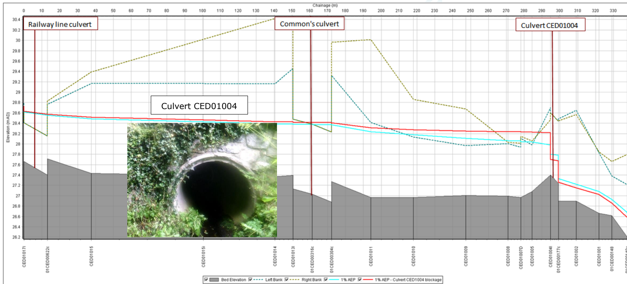
Figure D0-14: 1% AEP Longitudinal Section – Culvert CED1004 Blockage
