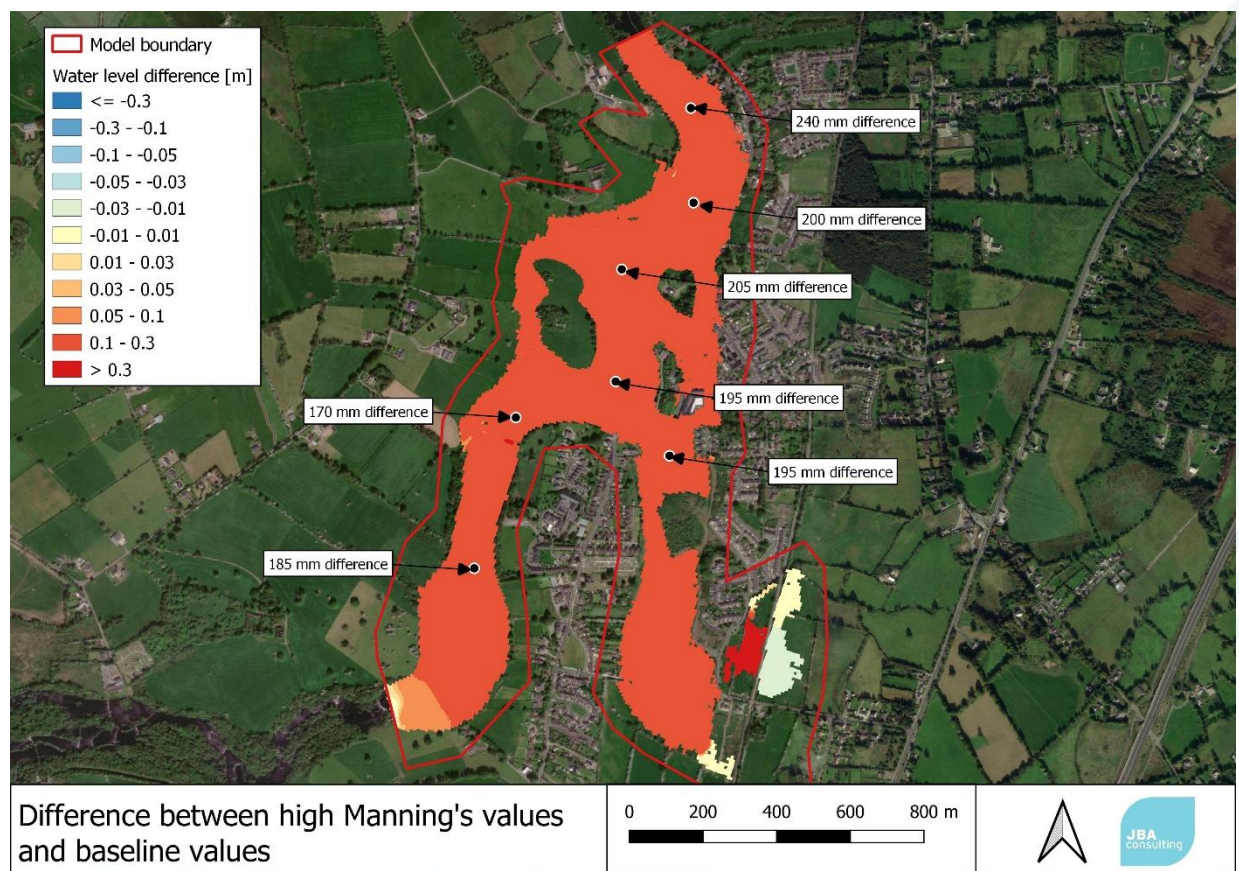
Figure 4-14: Difference between high Manning's n values and baseline scenario (high Manning's minus baseline values)
