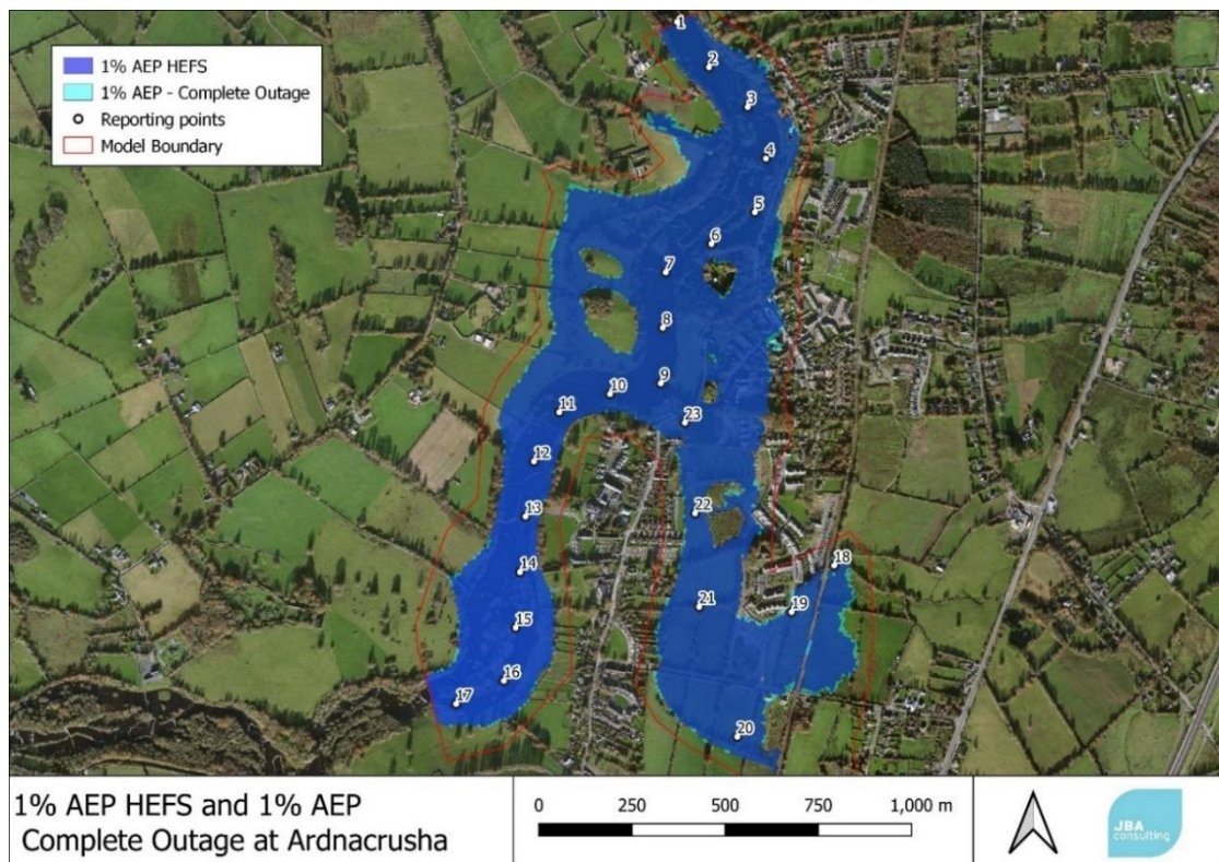
Figure B-15: 1% AEP HEFS for “504” event (standard operational conditions - 345 m 3 /s headrace flow) and 1% Complete Outage at Ardnacrusha (zero headrace flow)
