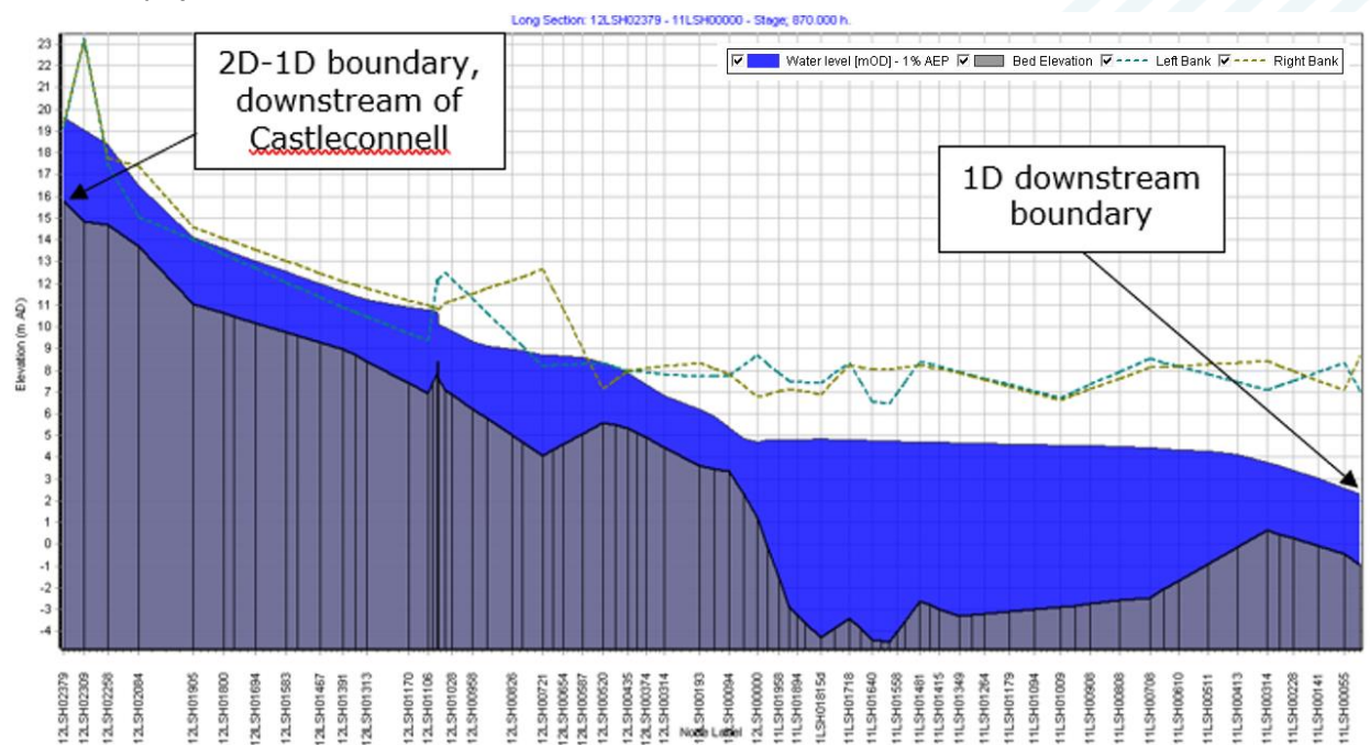
Figure 2-8: 1D model downstream of Castleconnell – Longitudinal Profile (1% AEP)
