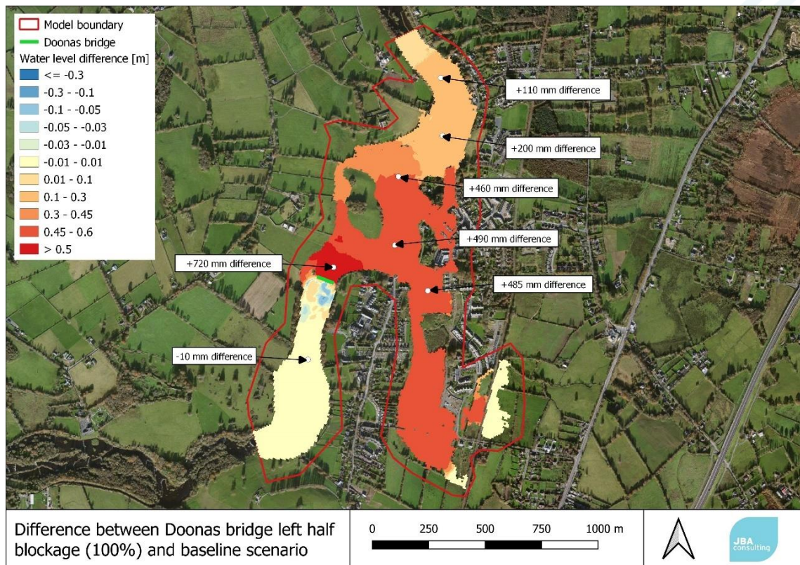
Figure 4-10: Difference between bridge blockage (left half, 100%) and baseline scenario (blockage scenario – baseline scenario)
