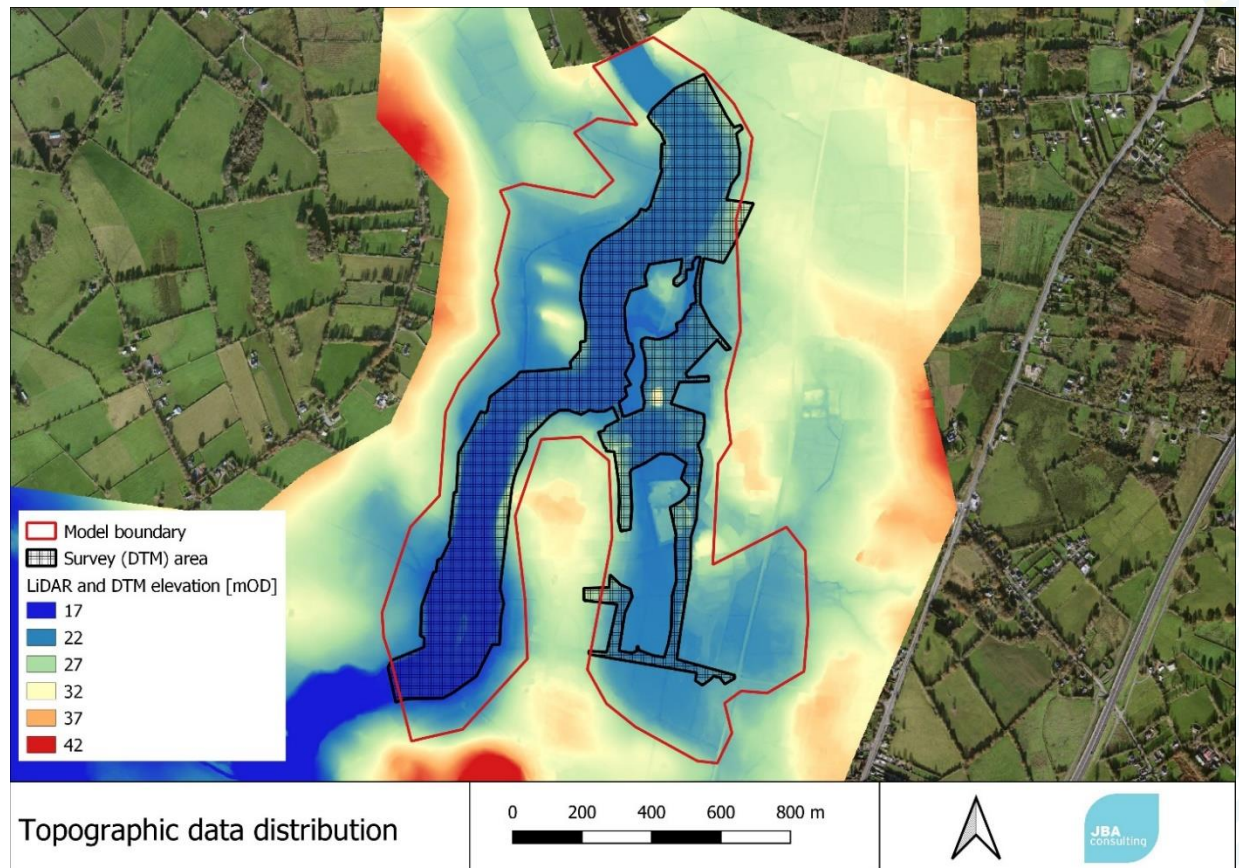
Figure 2-13: Topographic data distribution in the model
