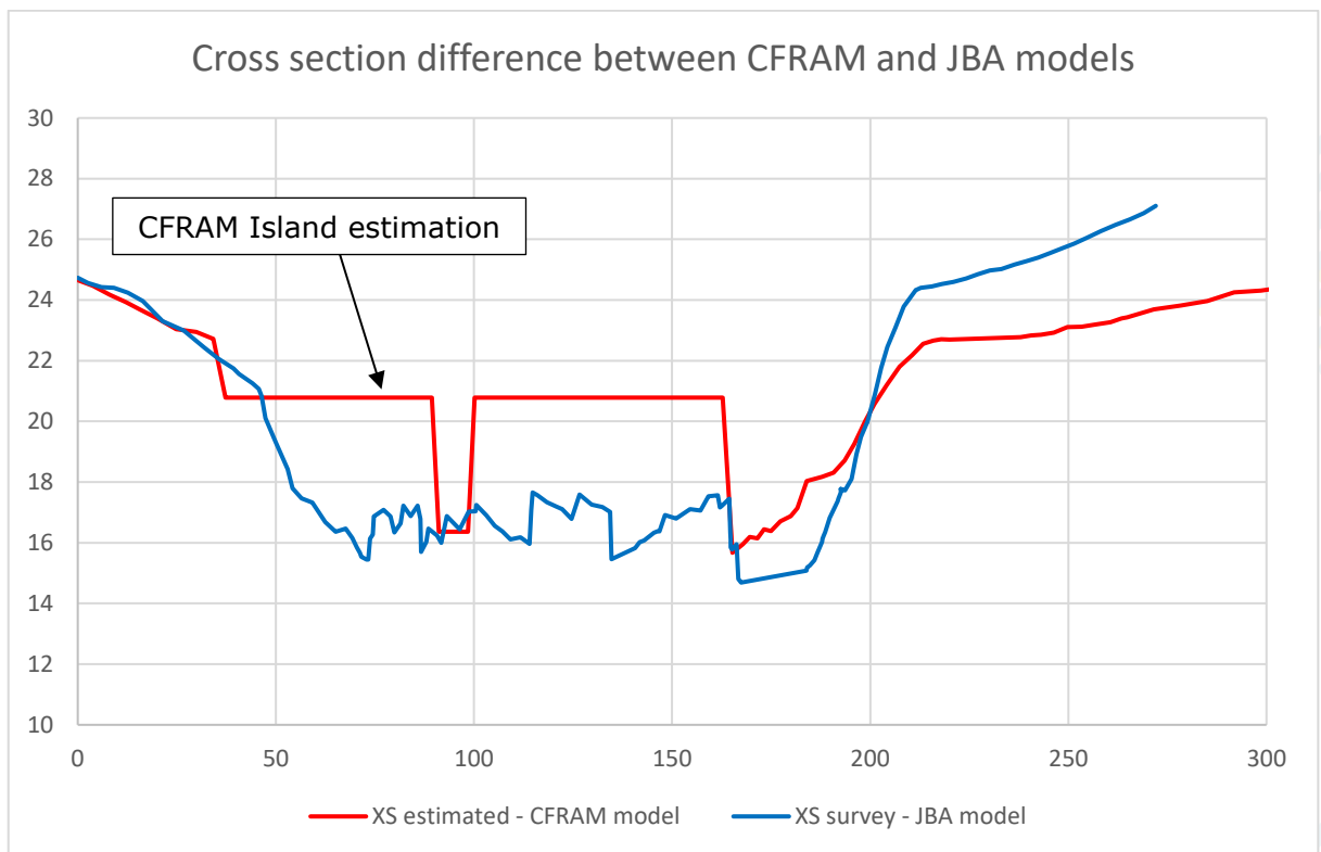
Figure 3-6: Cross section 12LSH02258 - Difference between CFRAM model and FRS model
