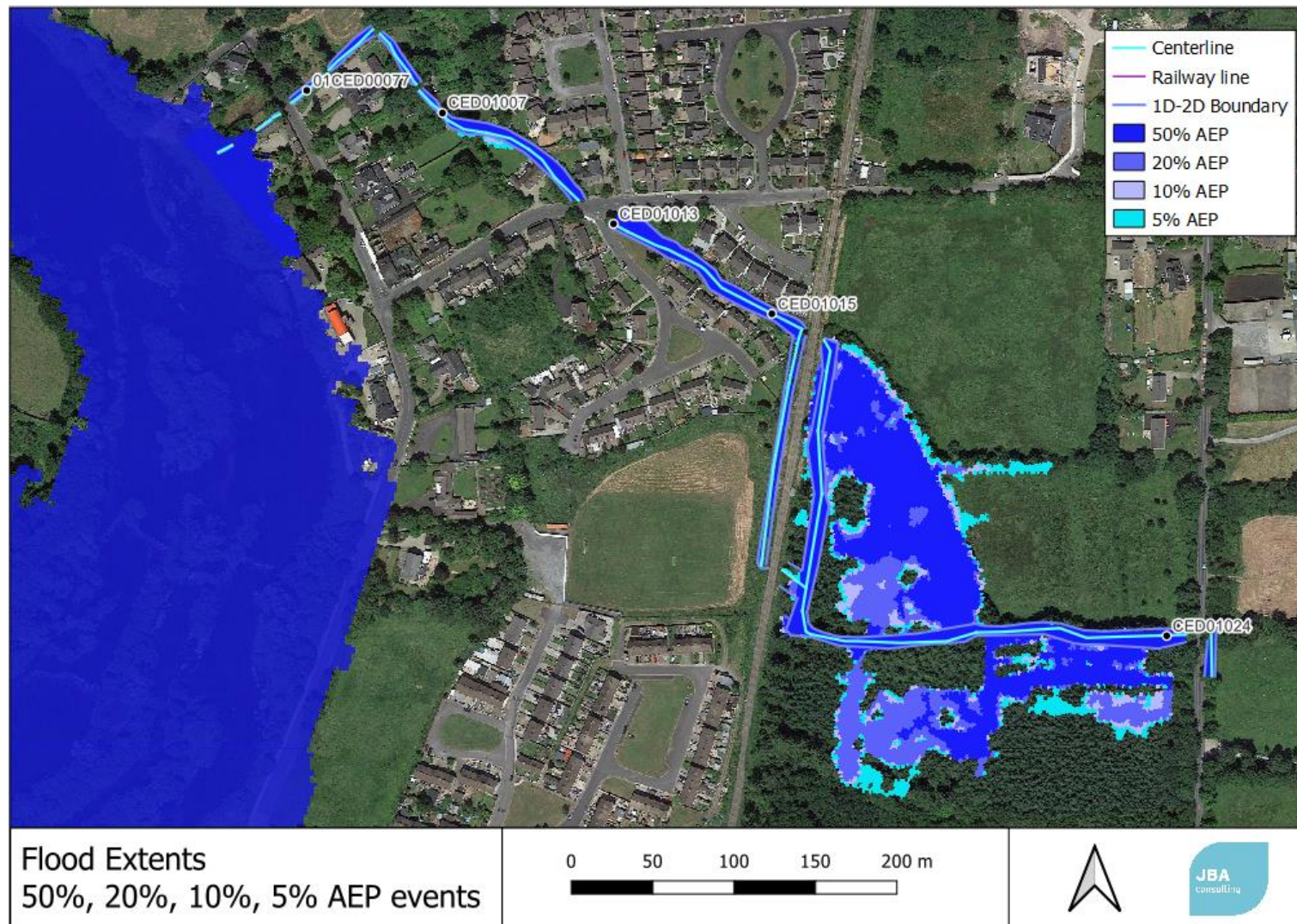
Figure D0-16: 50%, 20% 10%, 5% AEP Flood Extents
