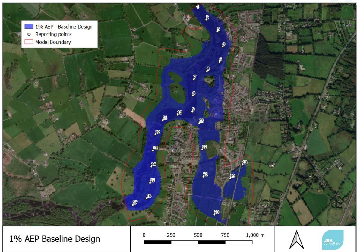
Figure 5-2: 1% AEP Baseline design event (258 m 3 /s headrace flow)
