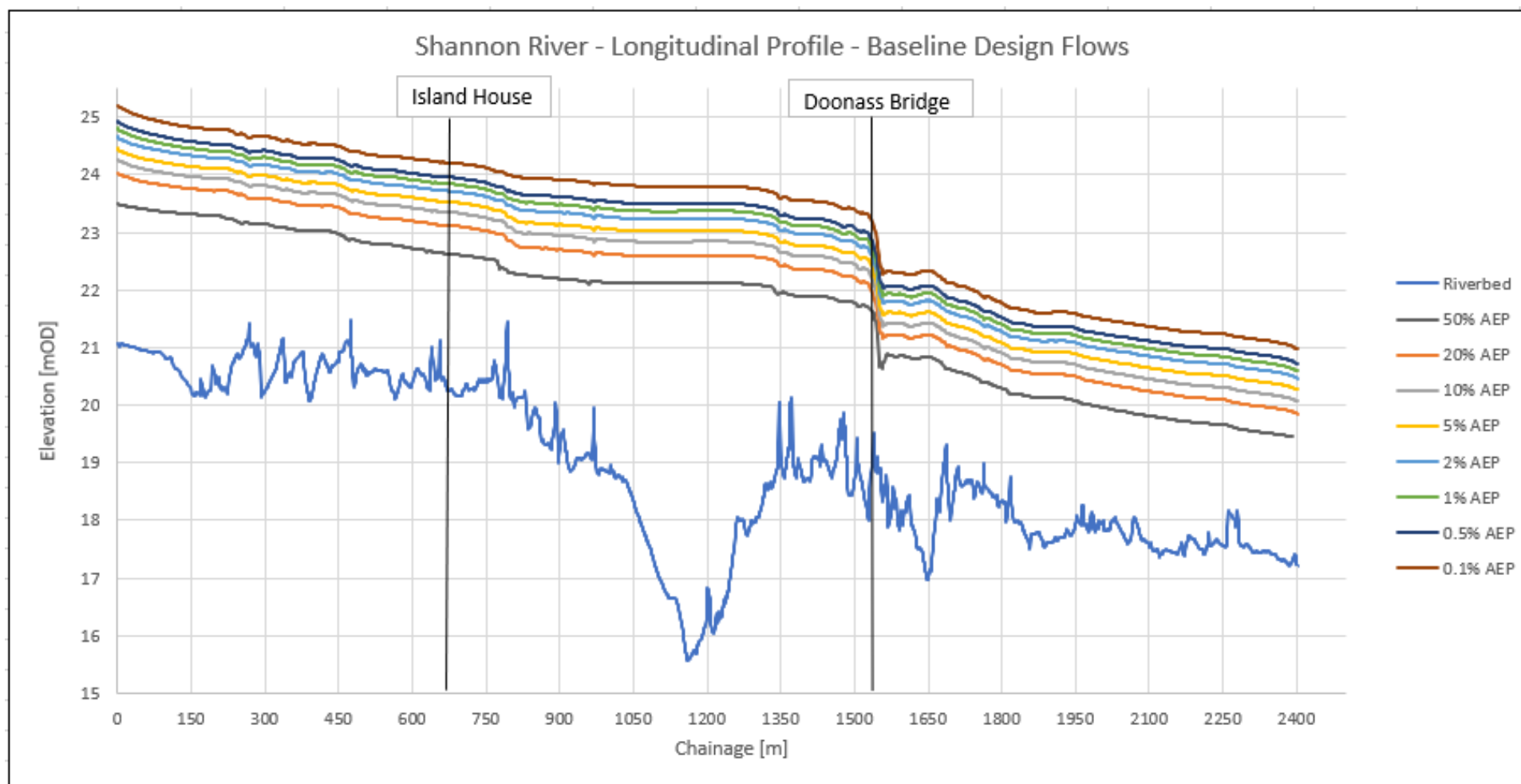
Figure B-11: Shannon River – Longitudinal Profile - Baseline Design Event (258 m 3 /s headrace flow)
