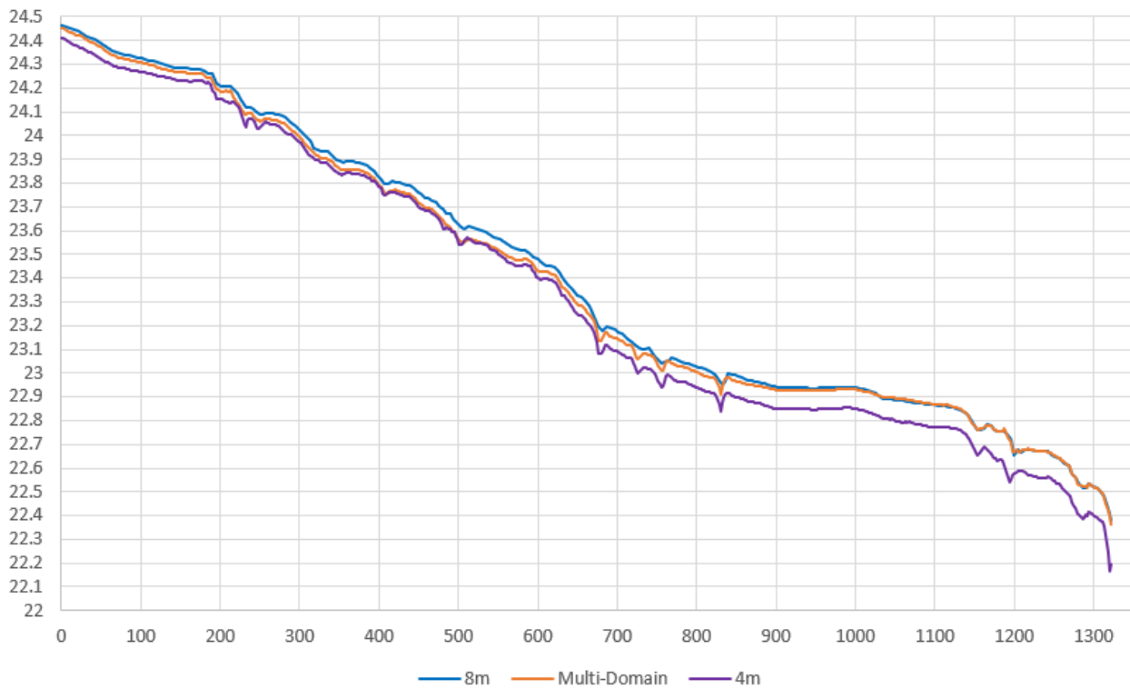
Figure 4-5: Longitudinal profile – Upstream of Doonass Bridge
