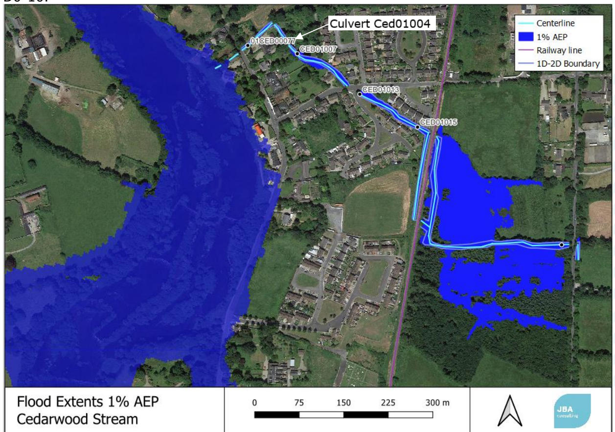
Figure D0-9: Cedarwood Stream – 1% AEP Flood Extent
