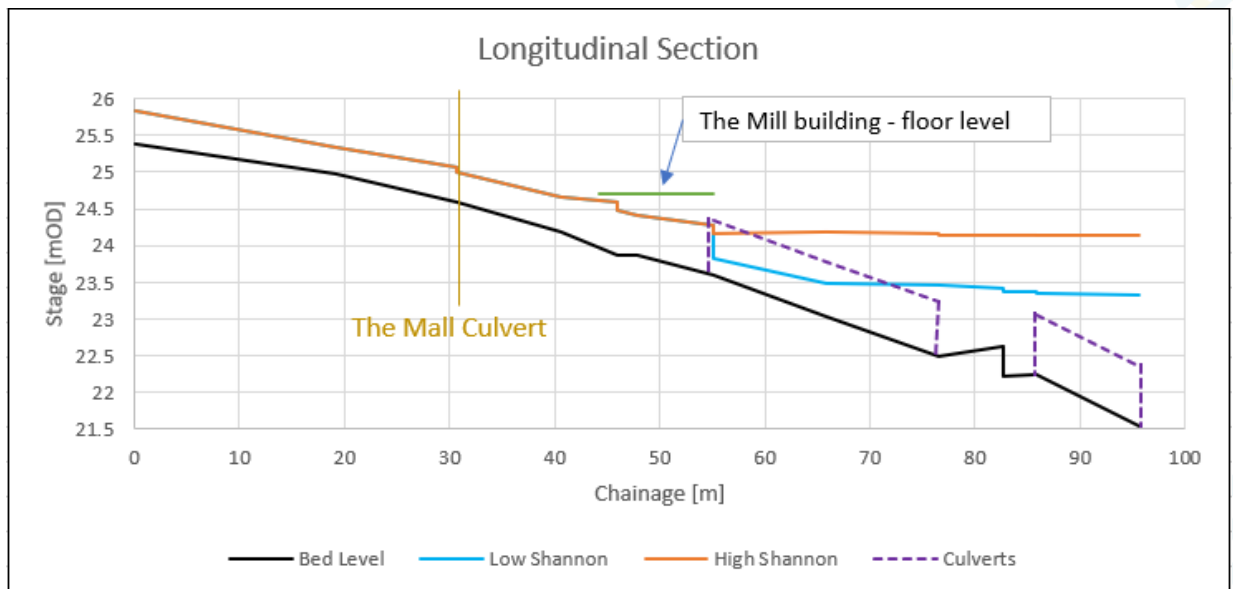
Figure D0-24: Longitudinal Section - Cedarwood Stream Downstream
