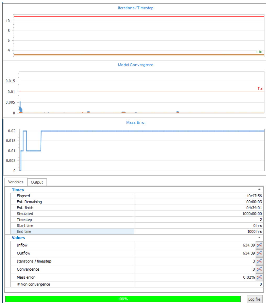
Figure 6-1: Flood Modeller stability plots – Shannon Model
