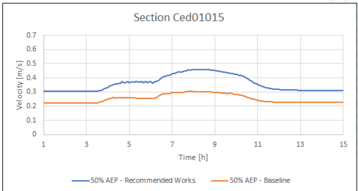
Figure D0-26: 50% AEP Velocities – Section Ced01015 (Downstream of railway line)
